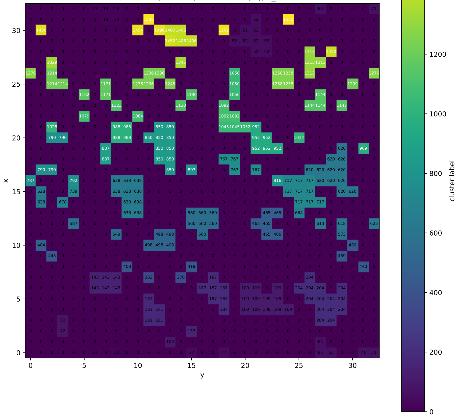
Cluster labels, PVA-100, T = 0.5 , T_{dot} = 10^{*(-5)} , T_{init} = 1.0 , z = 0
