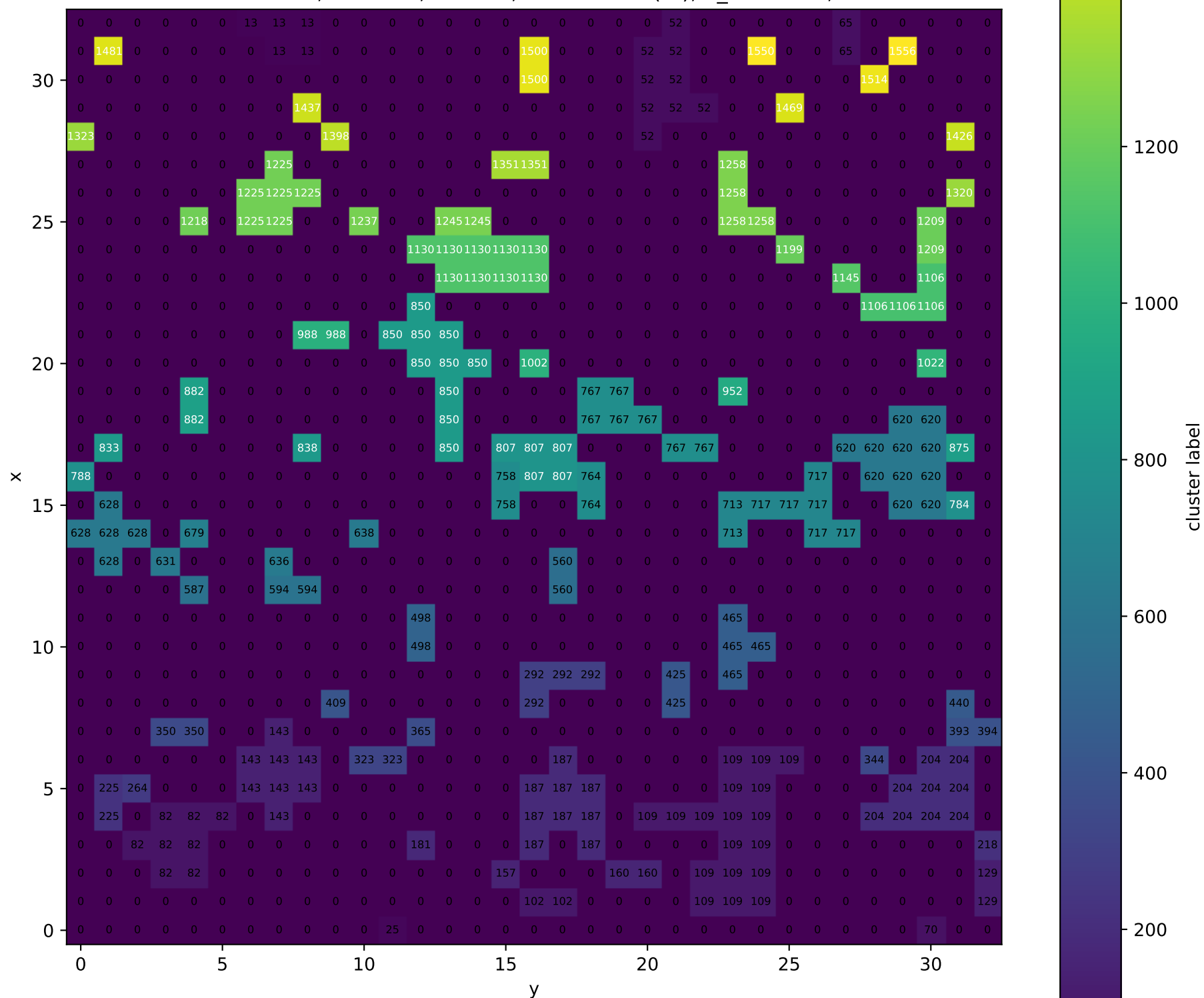
Cluster labels, PVA-100, T = 0.5 , T_{dot} = 10^{*(-5)} , T_{init} = 1.0 , z = 1
