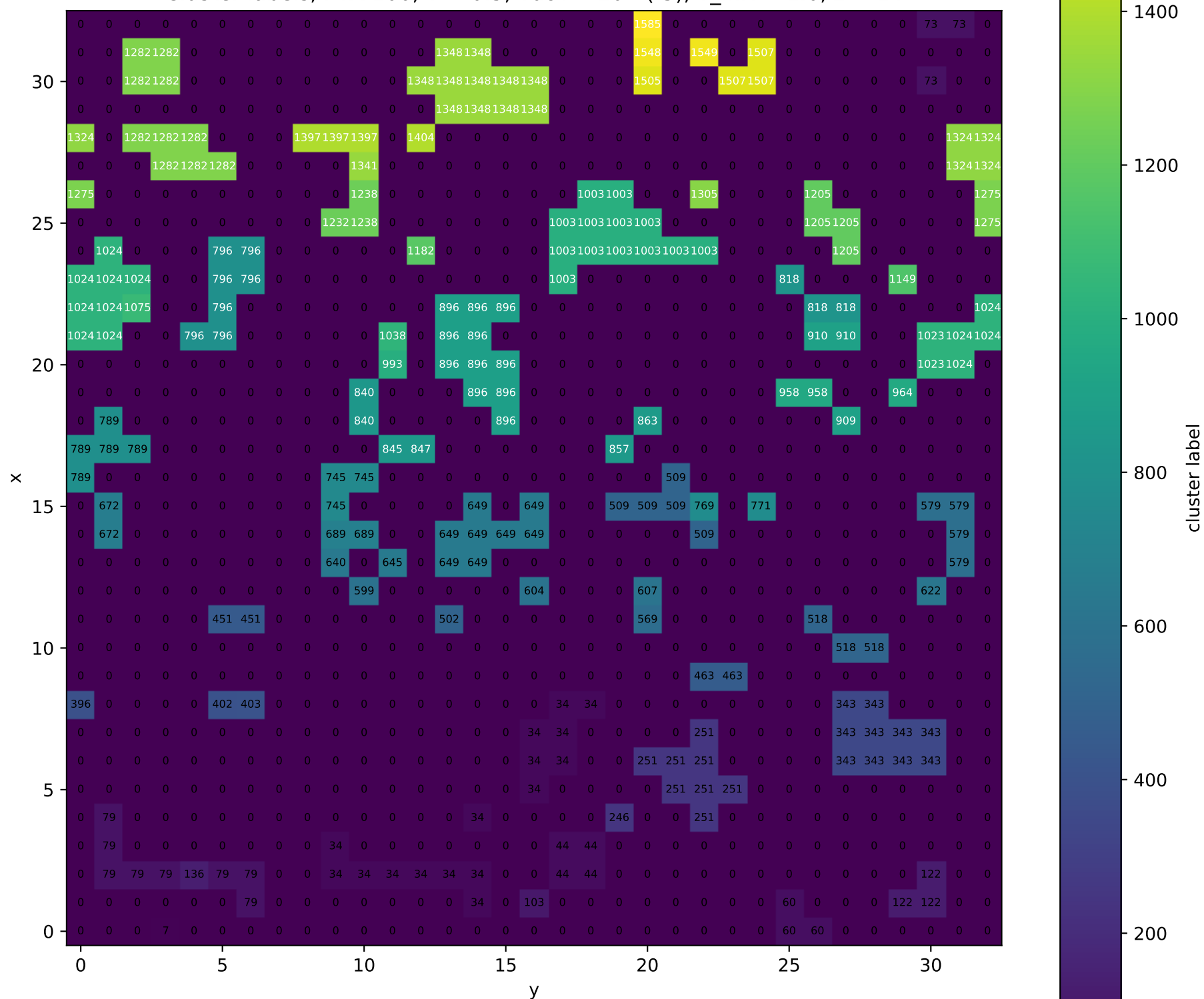
Cluster labels, PVA-100, T = 0.5 , T_{dot} = 10^{*(-5)} , T_{init} = 1.0 , z = 14
