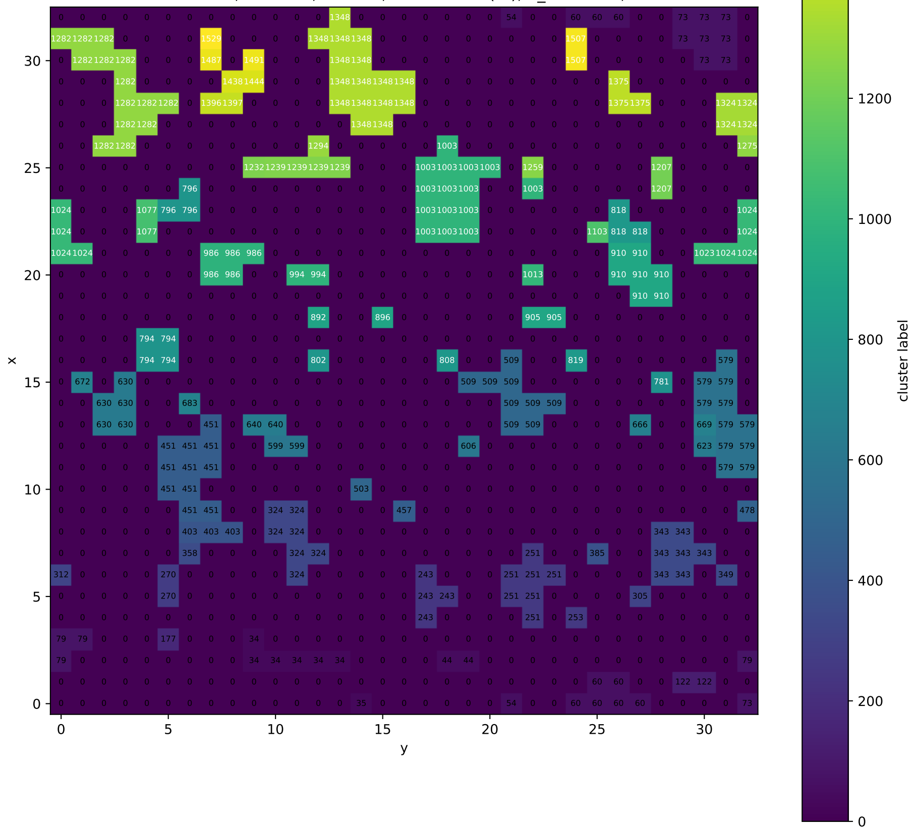
Cluster labels, PVA-100, T = 0.5 , T_{\text{dot}} = 10^{**}(-5) , T_{\text{init}} = 1.0 , z = 15
