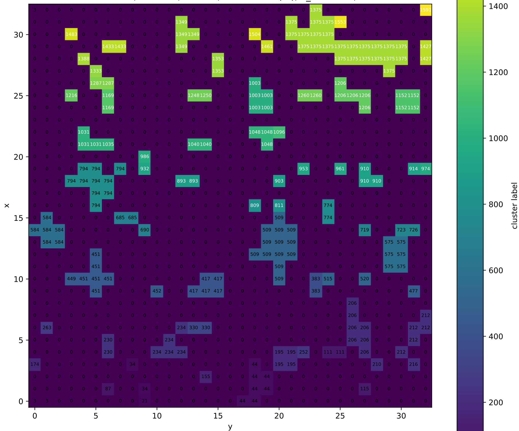
Cluster labels, PVA-100, T = 0.5 , T_{dot} = 10^{**}(-5) , T_{init} = 1.0 , z = 18
