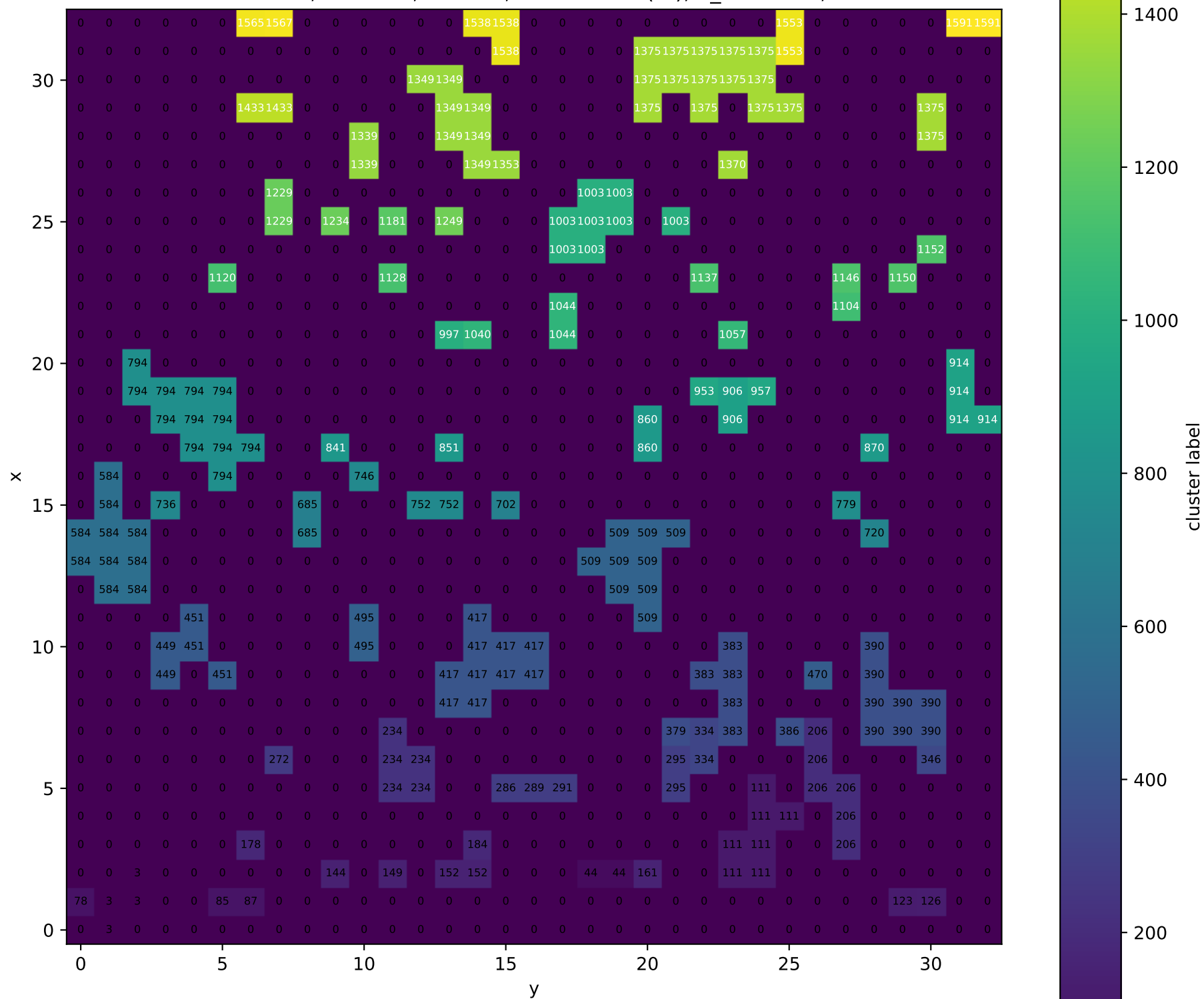
Cluster labels, PVA-100, T = 0.5 , T_{\text{dot}} = 10^{**}(-5) , T_{\text{init}} = 1.0 , z = 19
