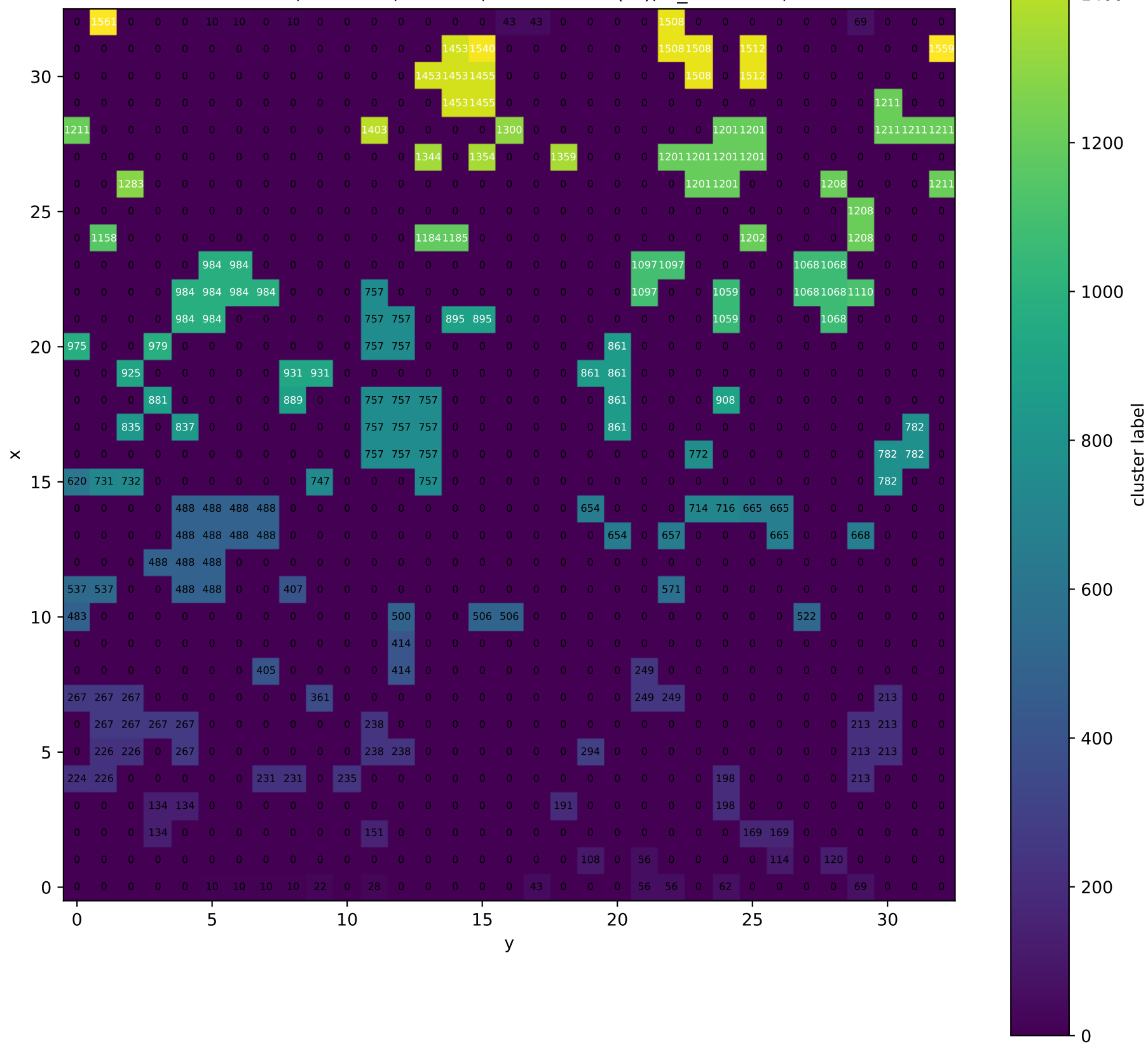
Cluster labels, PVA-100, T = 0.5 , T_{dot} = 10^{**}(-5) , T_{init} = 1.0 , z = 26
