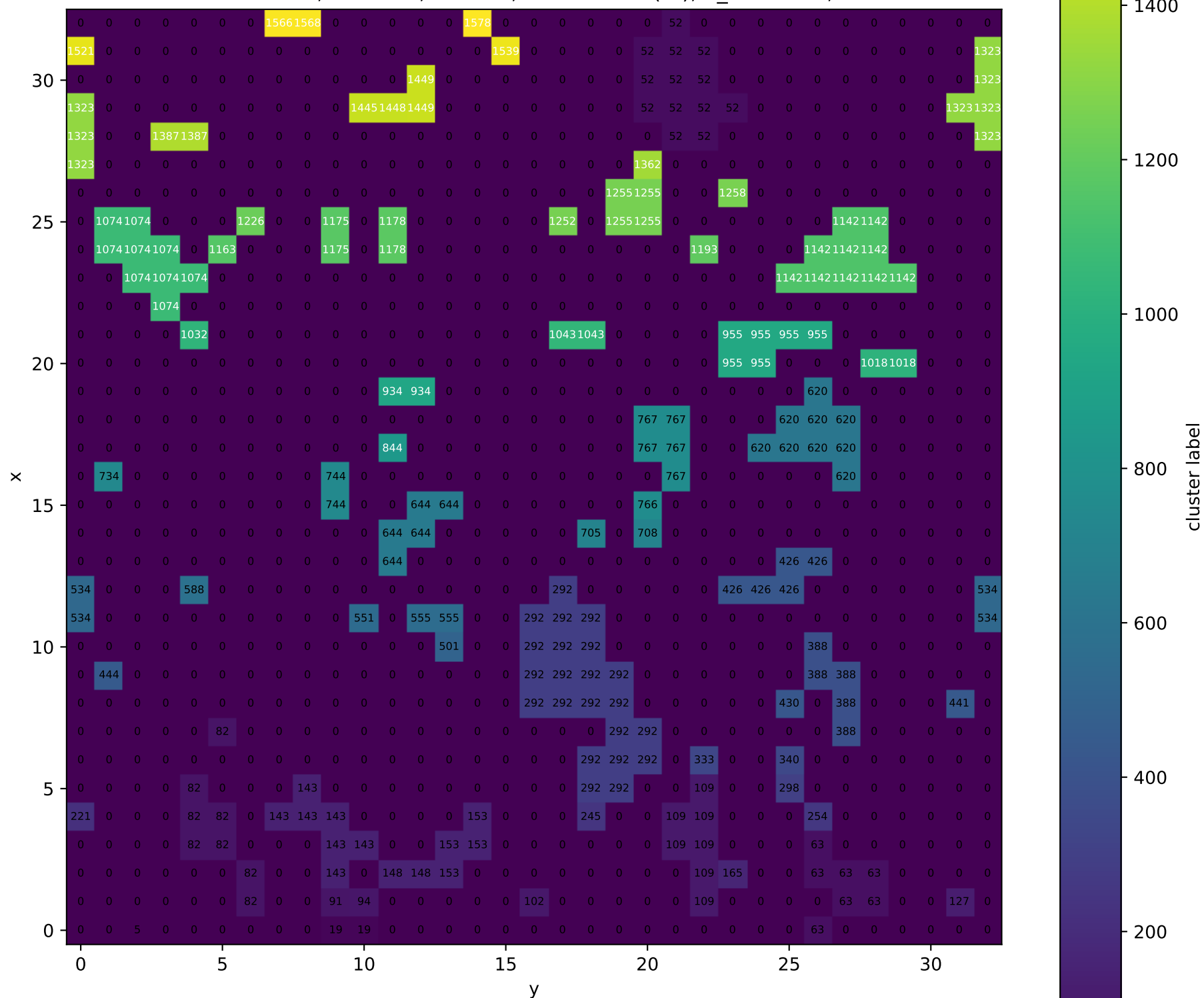
Cluster labels, PVA-100, T = 0.5 , T_{dot} = 10^{*(-5)} , T_{init} = 1.0 , z = 3
