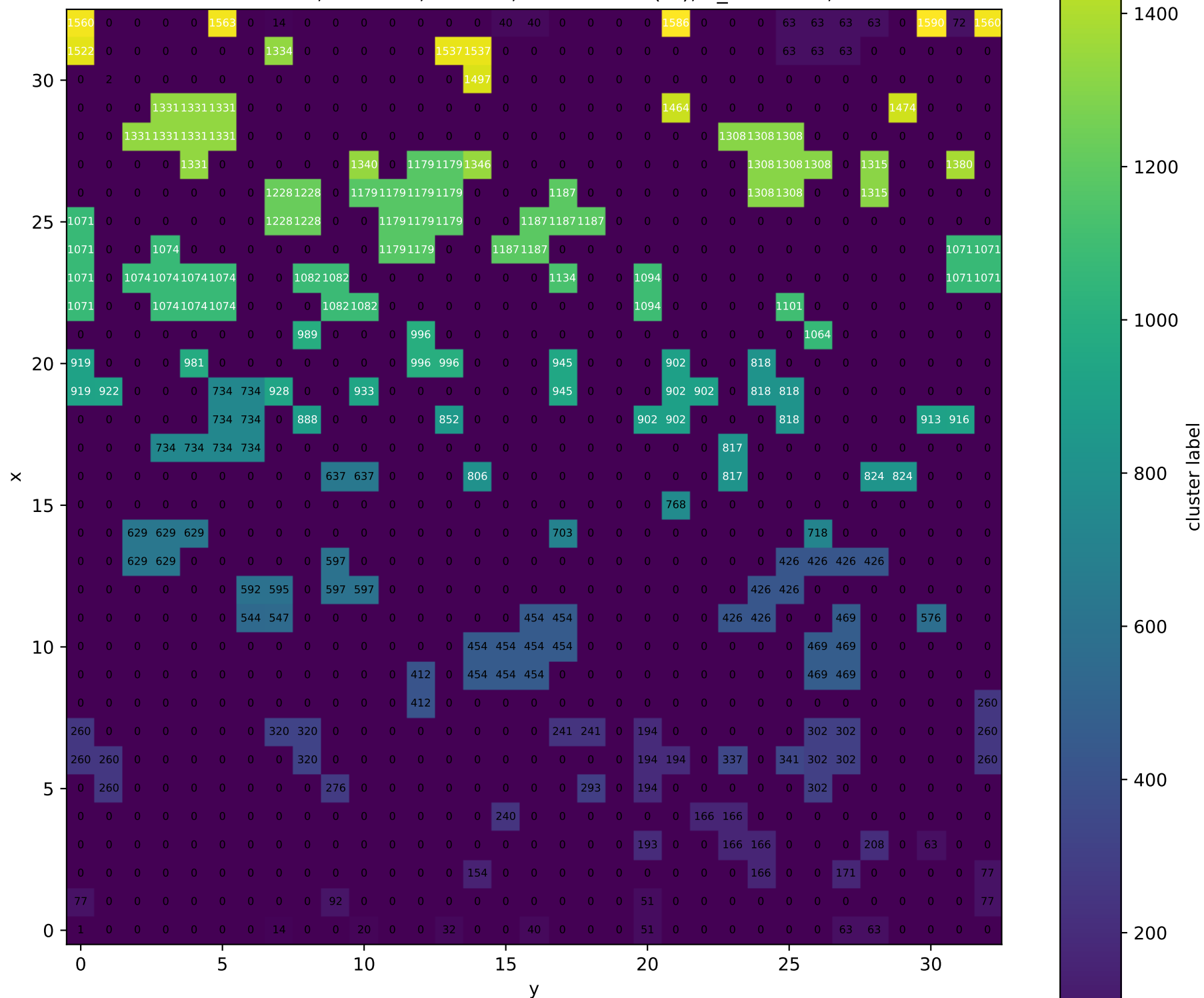
Cluster labels, PVA-100, T = 0.5 , T_{\text{dot}} = 10^{*(-5)} , T_{\text{init}} = 1.0 , z = 7
