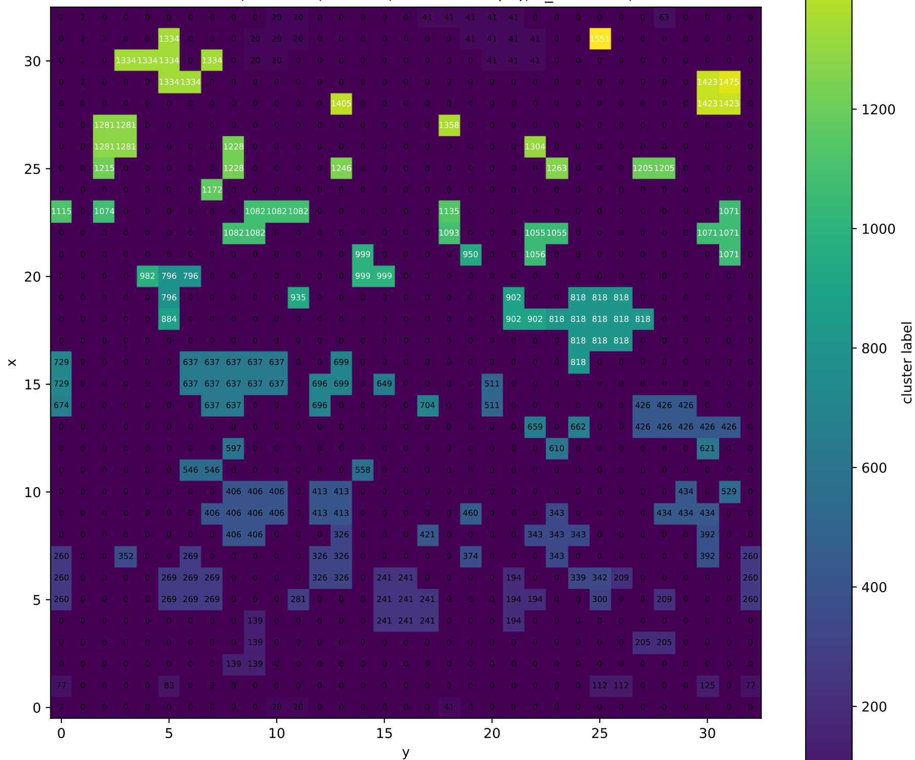
Cluster labels, PVA-100, T = 0.5 , T_{dot} = 10^{*(-5)} , T_{init} = 1.0 , z = 9
