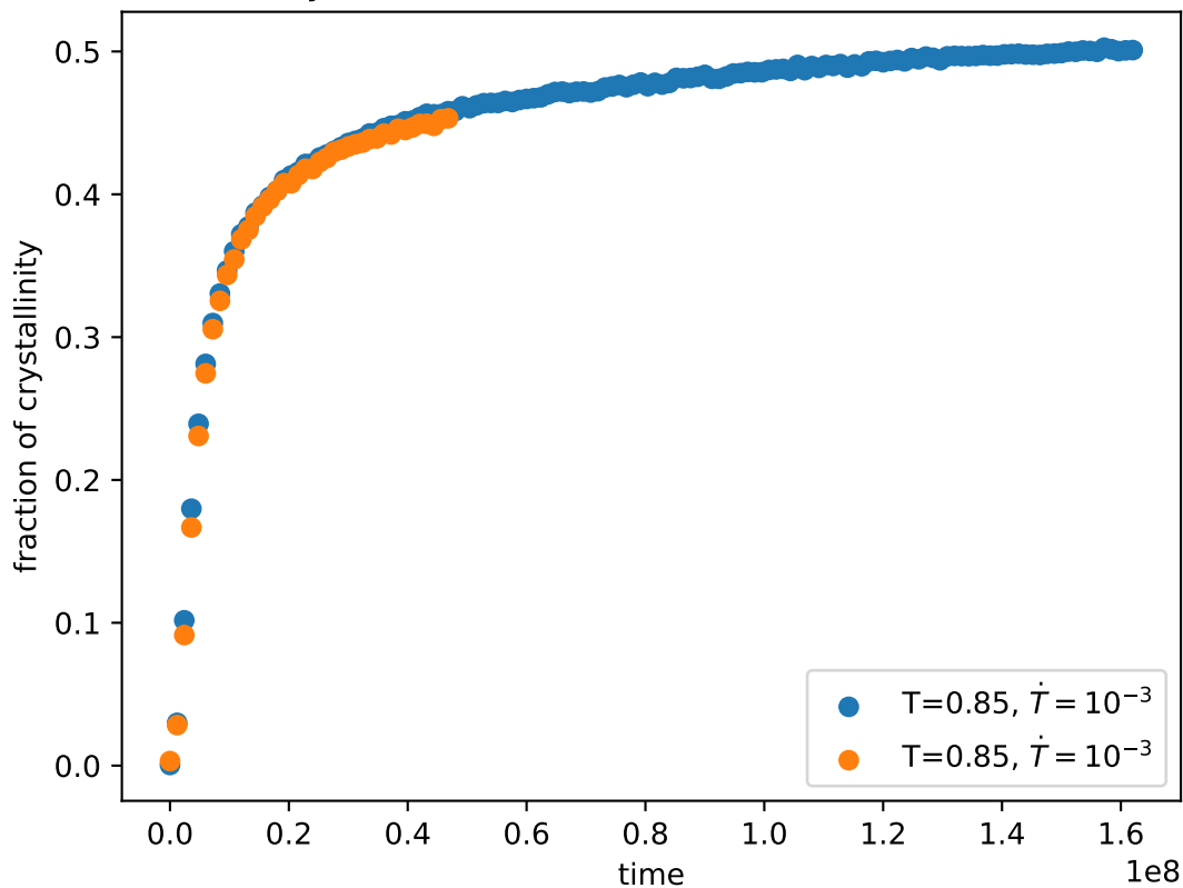
Crystallisation as function of time, PVA-100
