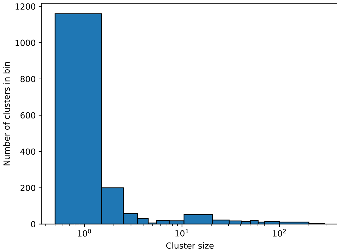
Crystalline domain size distribution, PVA-100, time 6000000, \phi = 0.277
