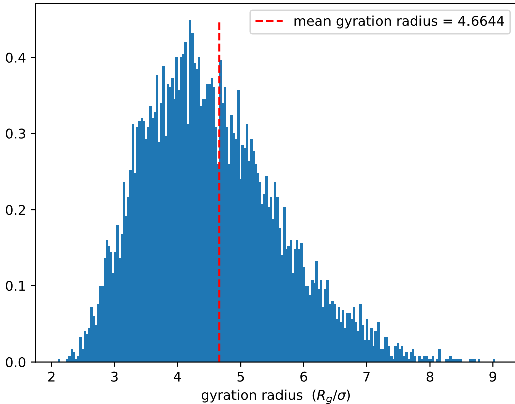
Distribution of the gyration radius, PVA-100, simulation start
