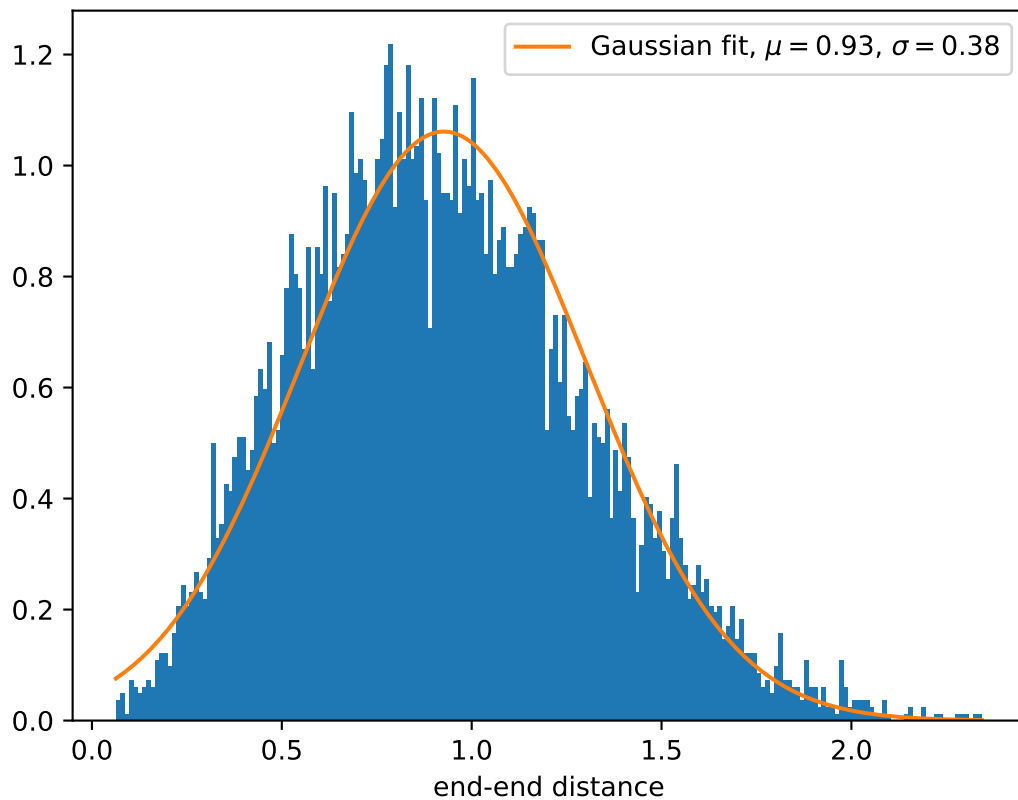
Distribution of end-to-end distance, PVA-100, simulation start
