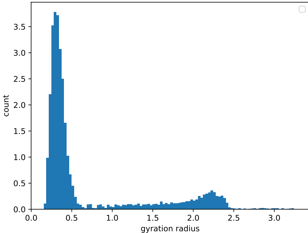
Distribution of the gyration radius, PVA-100, simulation start
