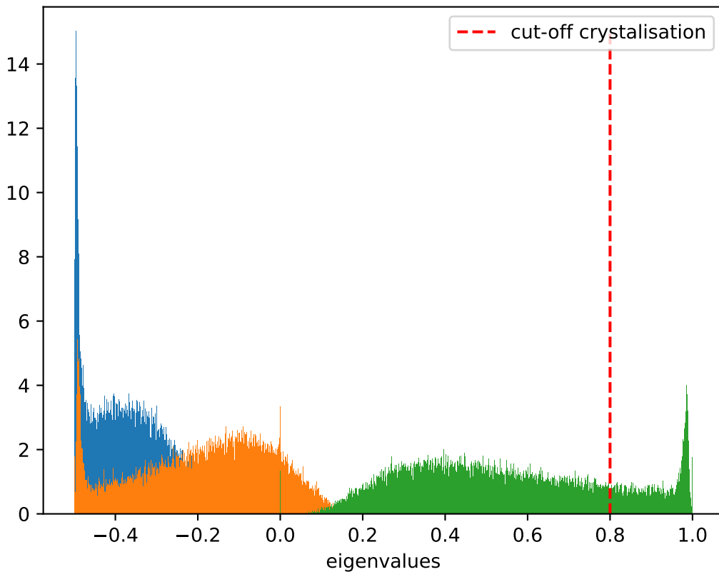
Distribution of eigenvalues at T = 0.625 , \dot{T} = 10^{-7}
