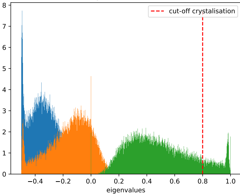
Distribution of eigenvalues at T = 0.775 , \dot{T} = 10^{-7}
