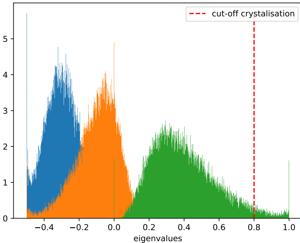
Distribution of eigenvalues at T = 0.85 , \dot{T} = 10^{-7}
