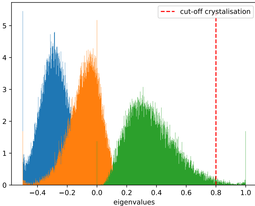
Distribution of eigenvalues at T = 0.875 , \dot{T} = 10^{-7}
