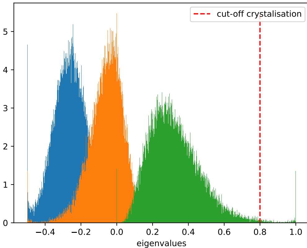
Distribution of eigenvalues at T = 0.95 , \dot{T} = 10^{-7}
