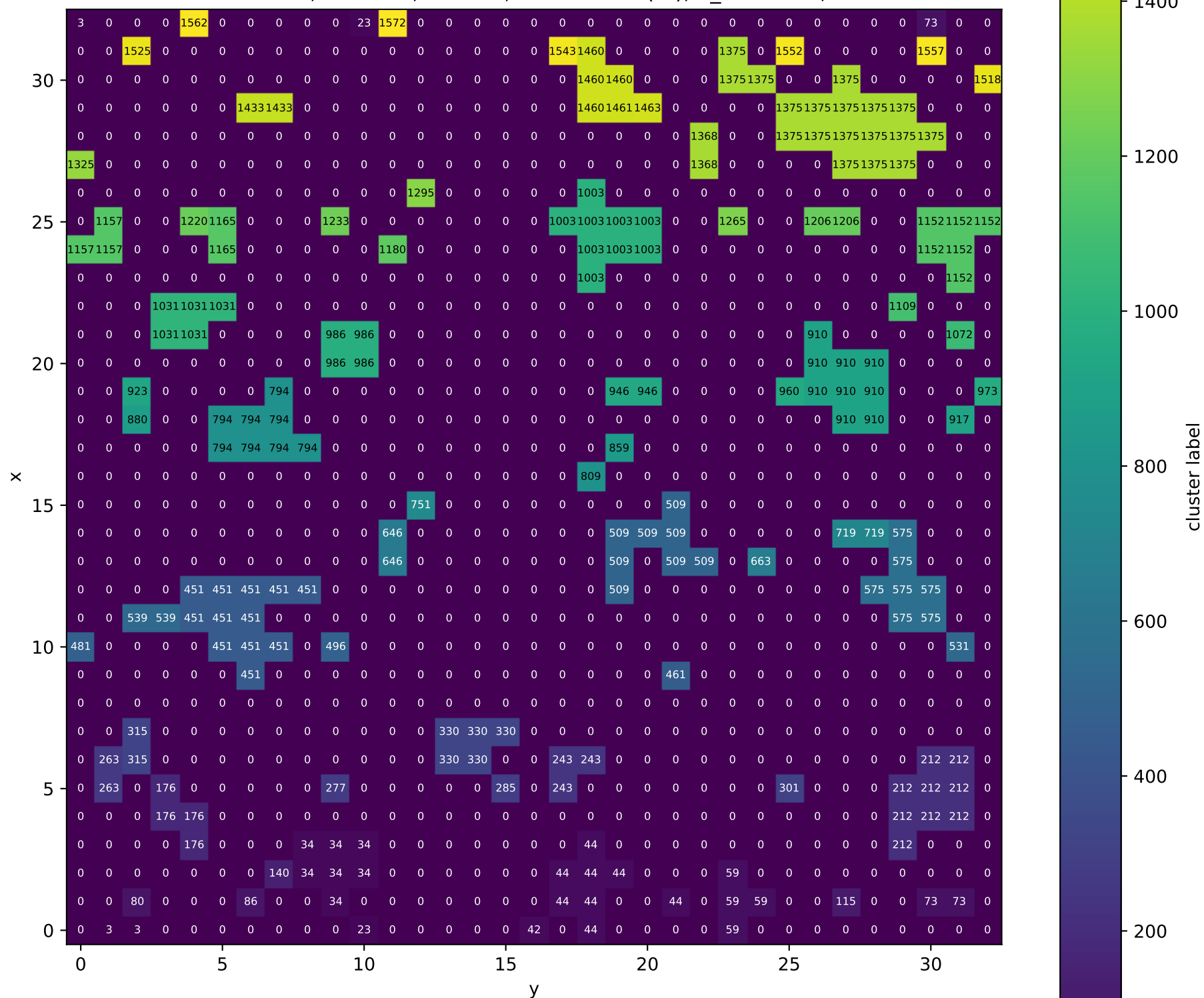
Cluster labels, PVA-100, T = 0.5 , T_{\text{dot}} = 10^{**}(-5) , T_{\text{init}} = 1.0 , z = 17
