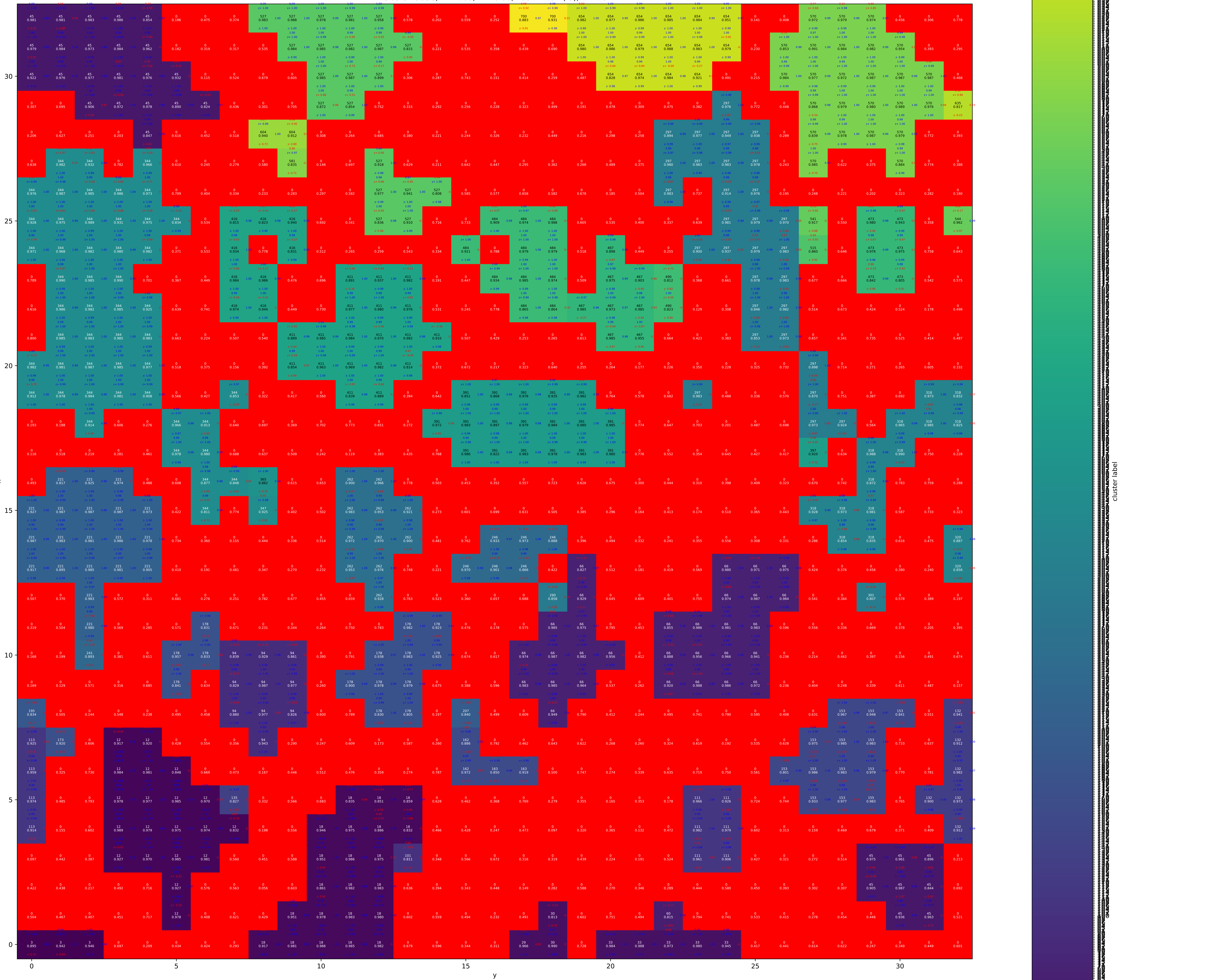
Cluster labels, PVA-100, T = 0.88, Tdot = 10**(-3), z = 10
