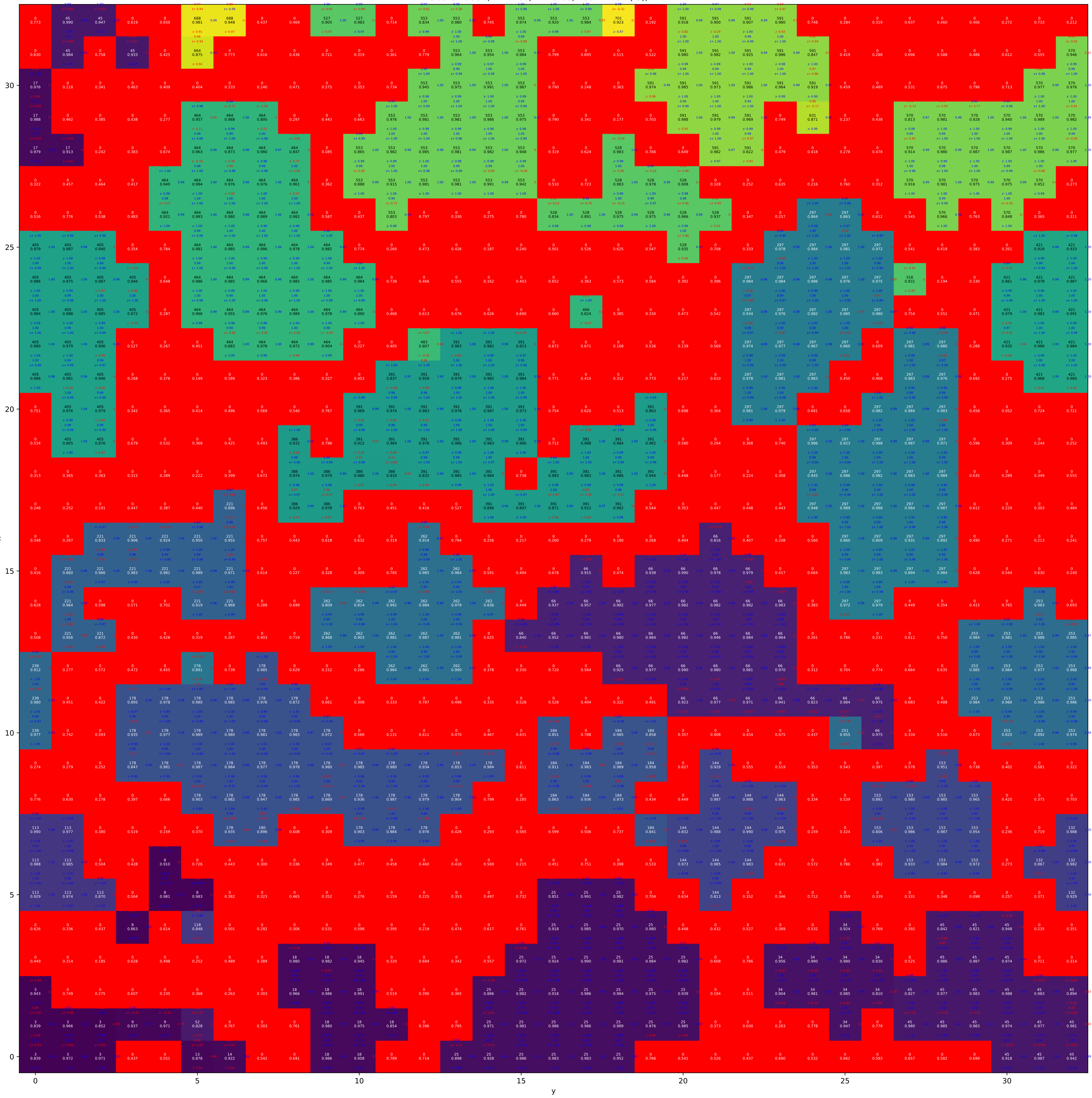
Cluster labels, PVA-100, T = 0.88, Tdot = 10**(-3), z = 14
