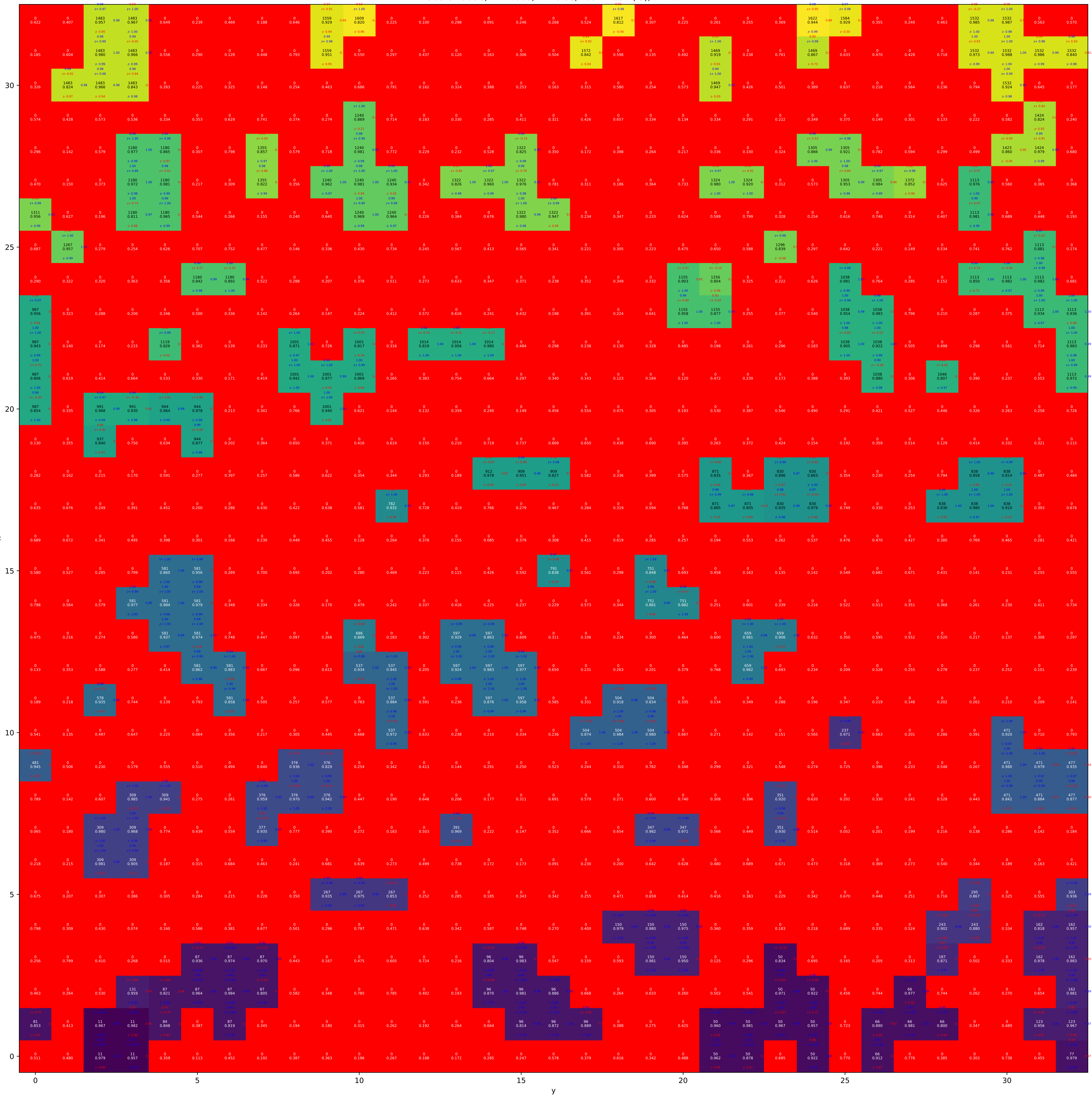
Cluster labels, PVA-1000, T = 0.88, Tdot = 10*(-3), z = 11
