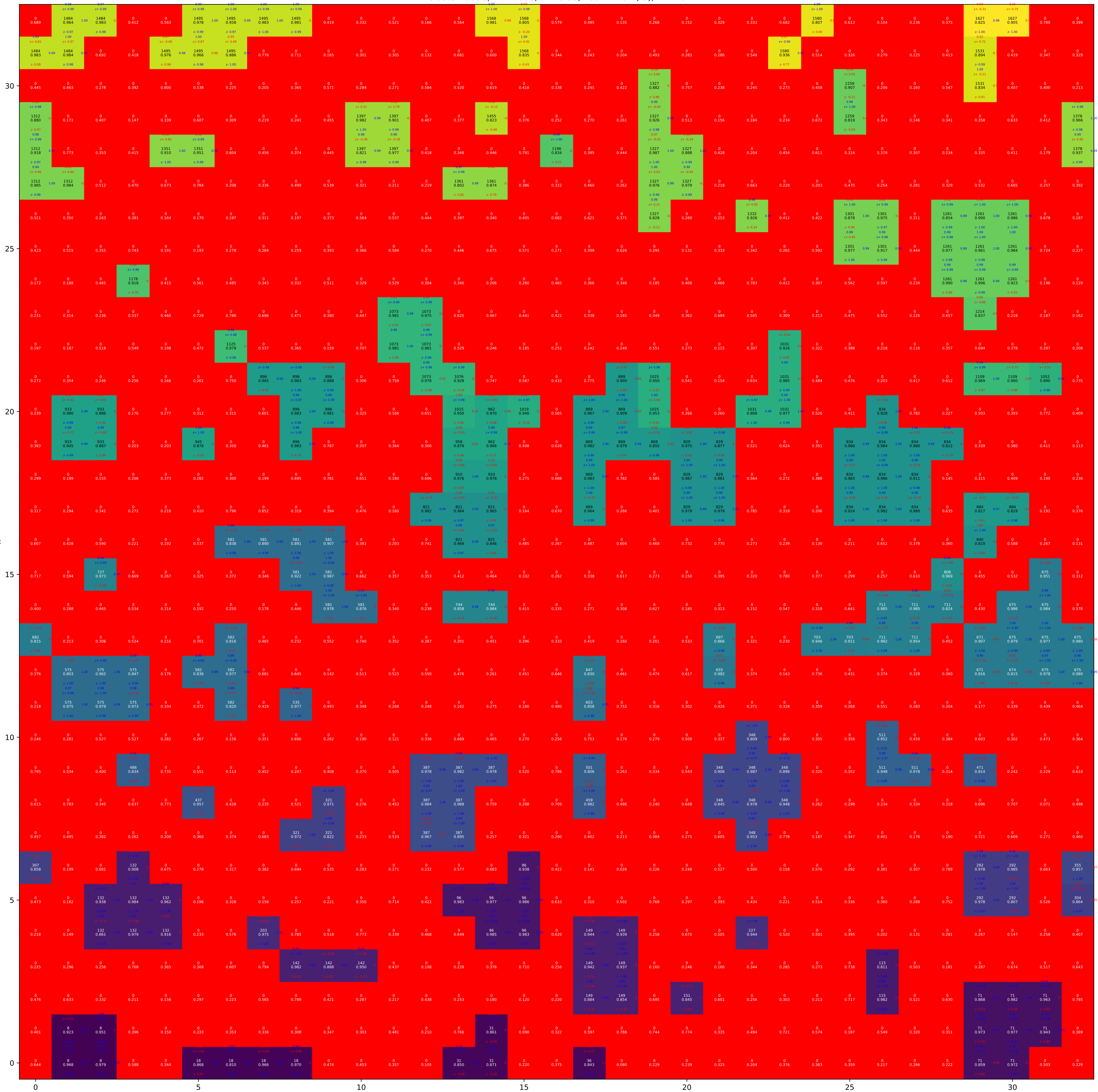
Cluster labels, PVA-1000, T = 0.88, Tdot = 10**(-3), z = 16
