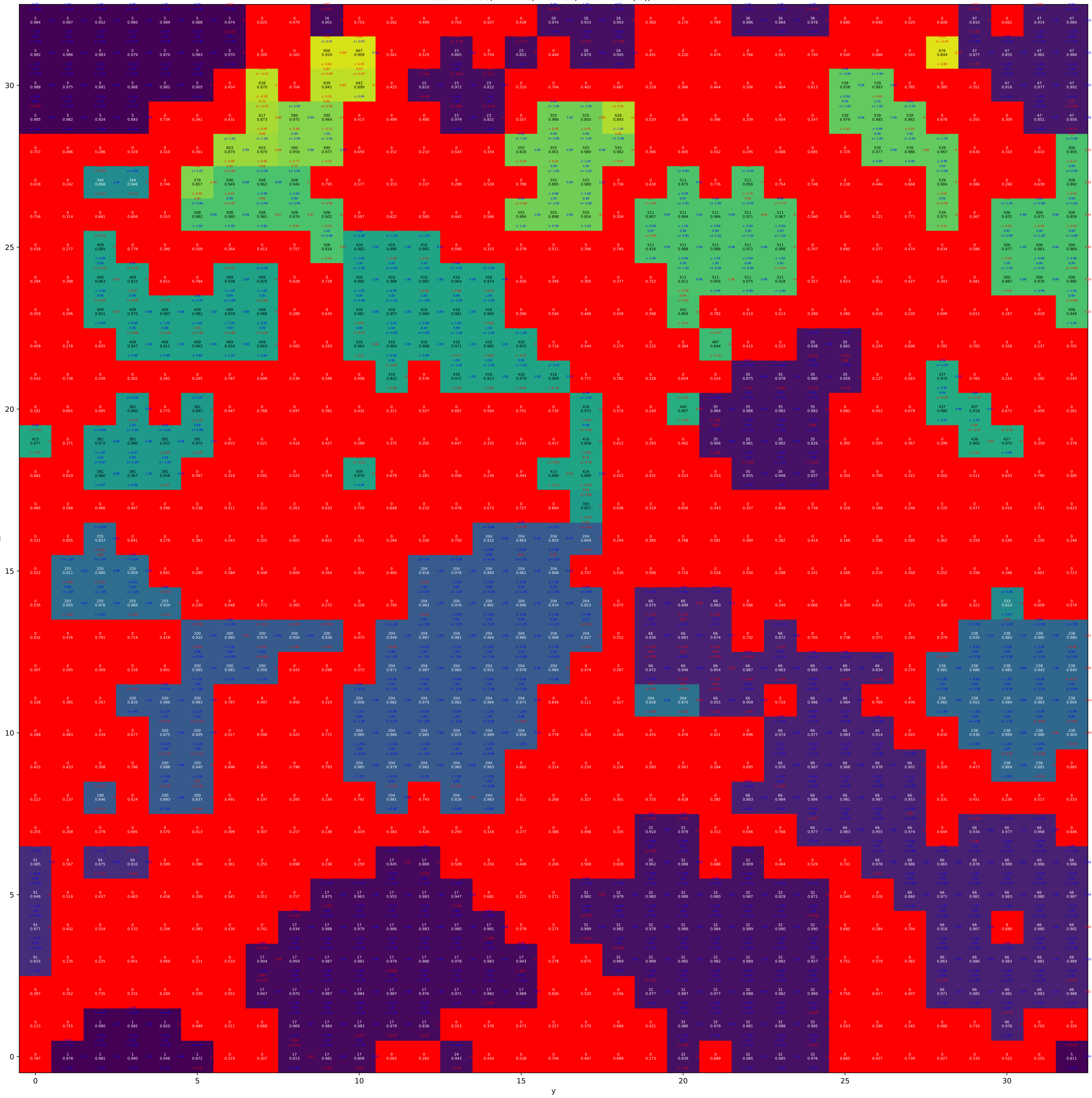
Cluster labels, PVA-100, T = 0.88, Tdot = 10*(-3), z = 0
