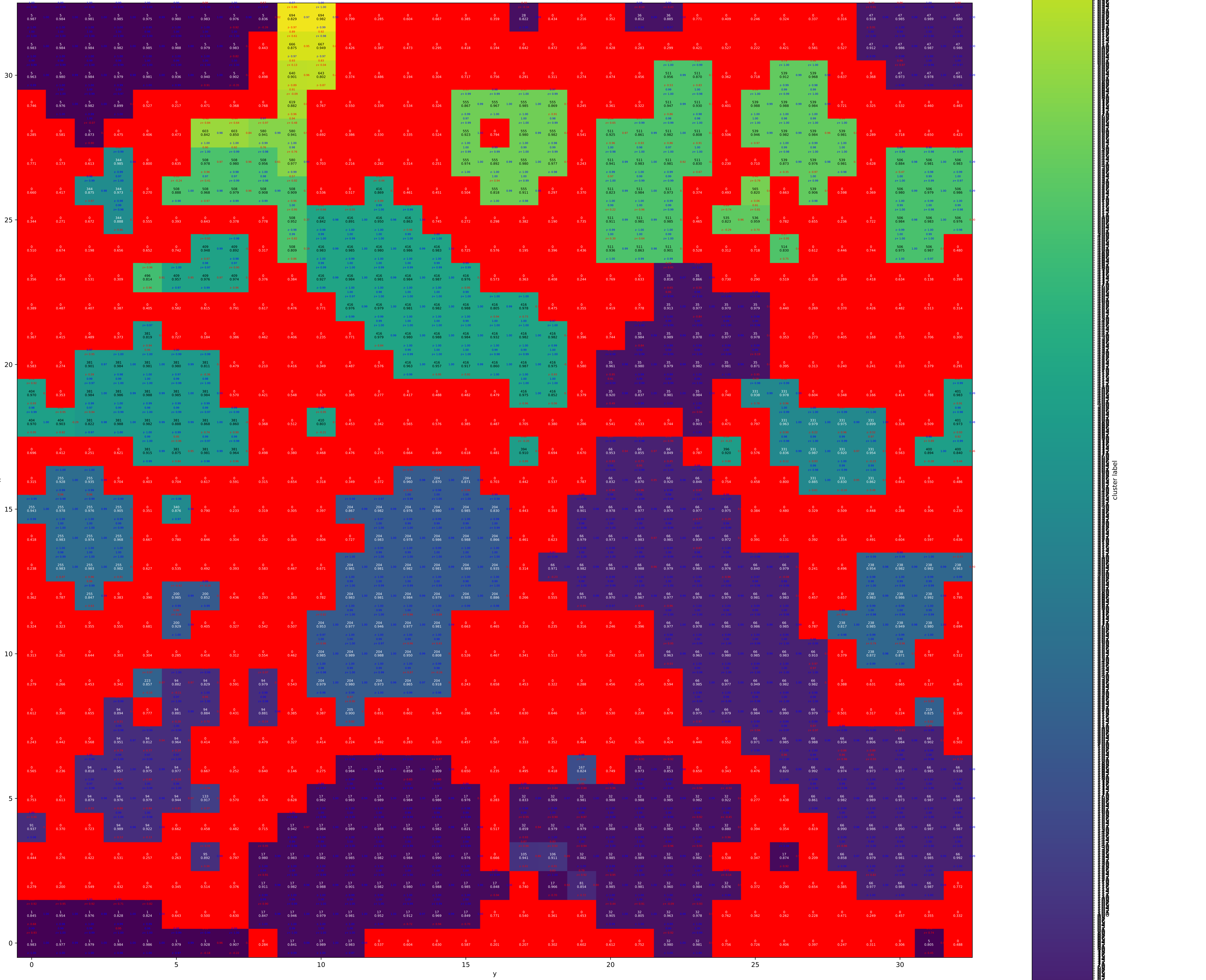
Cluster labels, PVA-100, T = 0.88, Tdot = 10**(-3), z = 1
