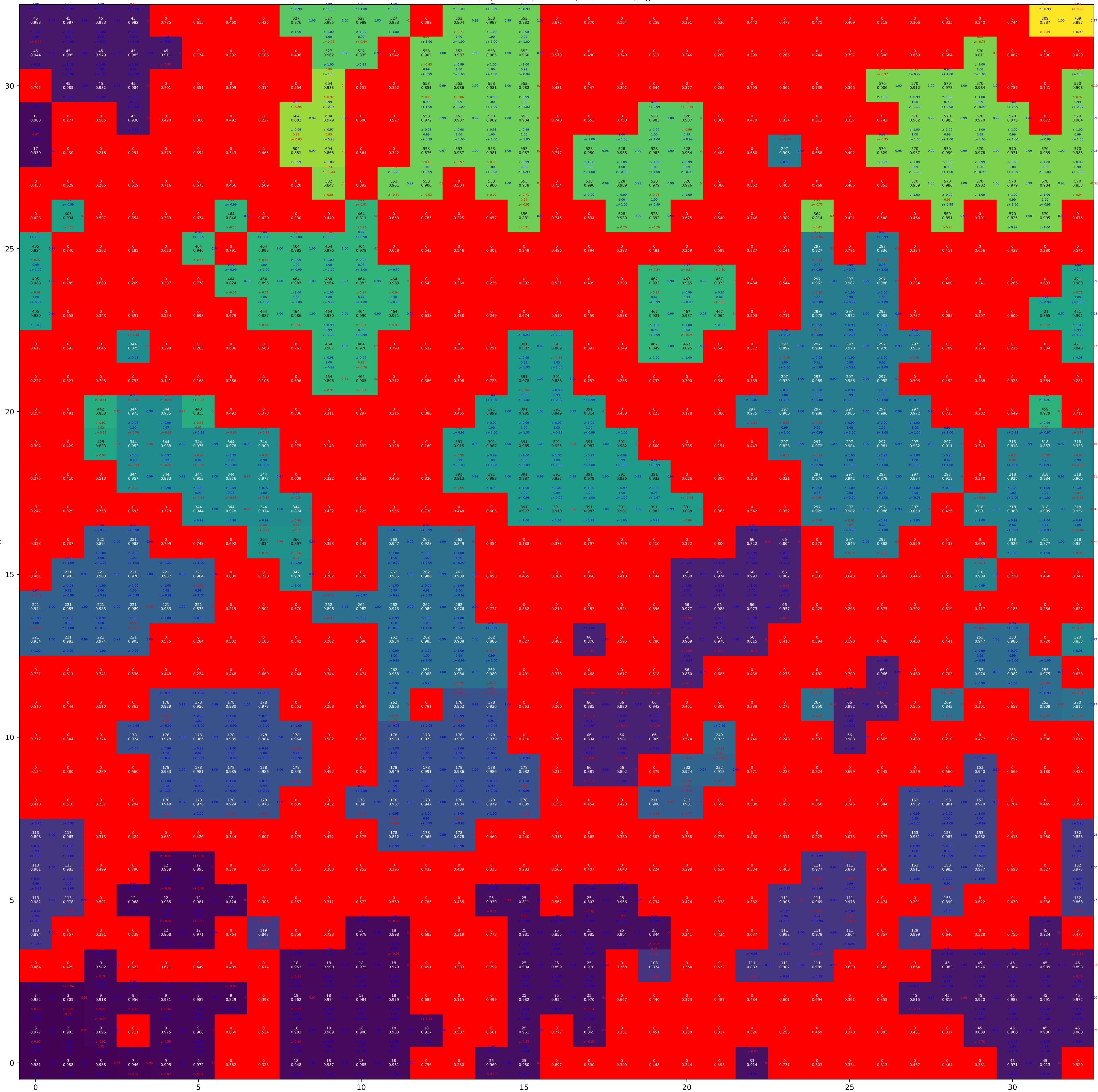
Cluster labels, PVA-100, T = 0.88, Tdot = 10**(-3), z = 12
