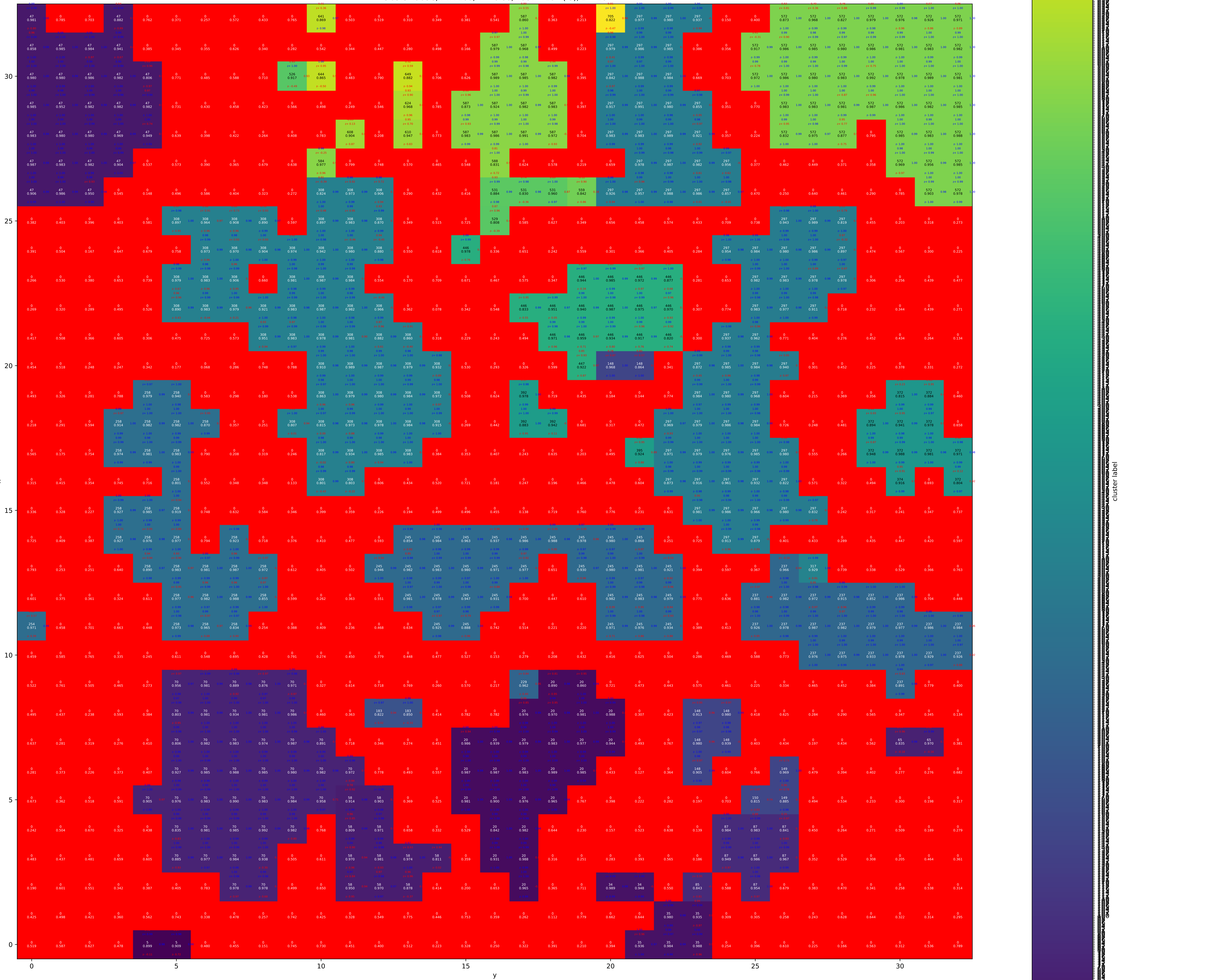
Cluster labels, PVA-100, T = 0.88, Tdot = 10**(-3), z = 26
