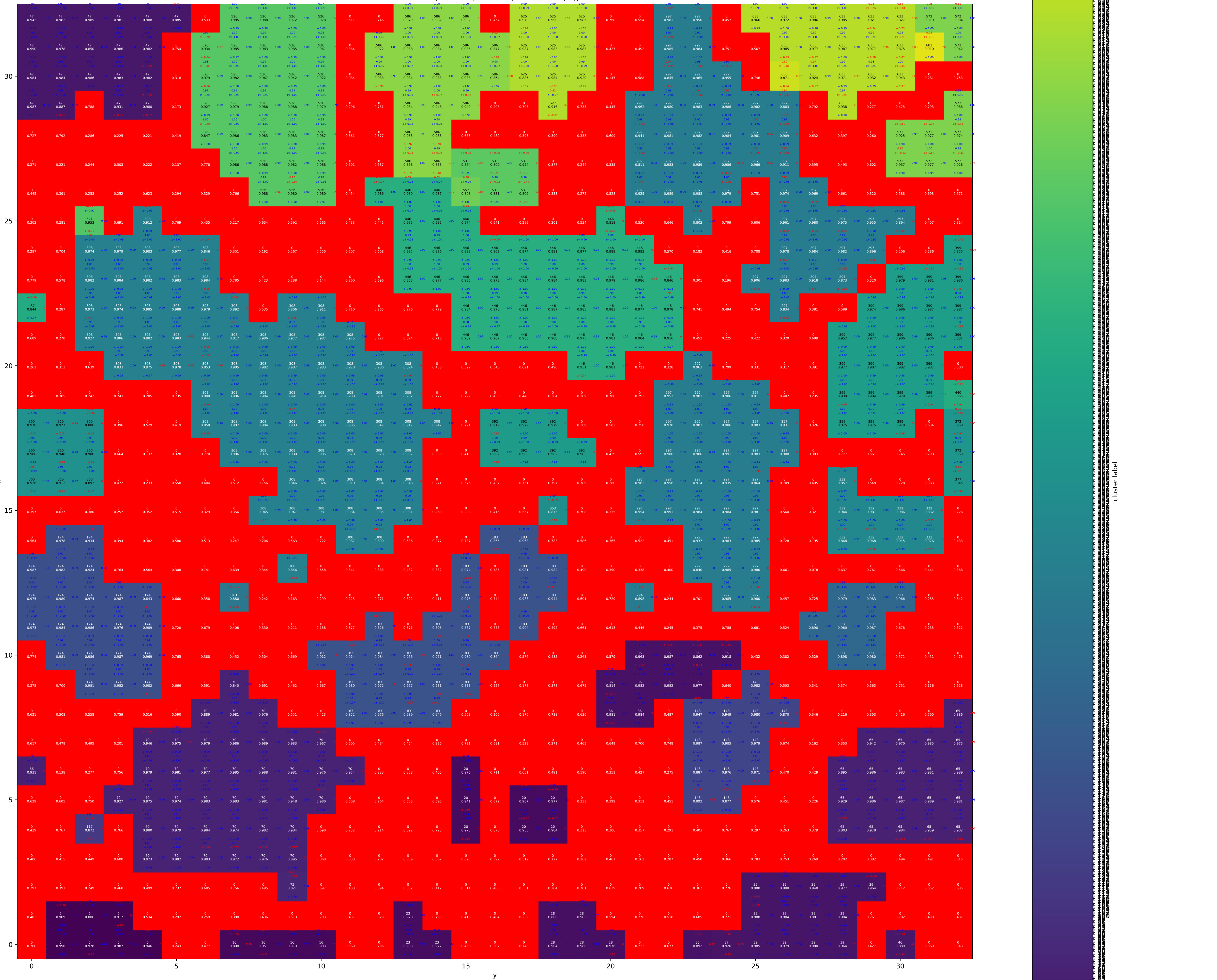
Cluster labels, PVA-100, T = 0.88, Tdot = 10**(-3), z = 29
