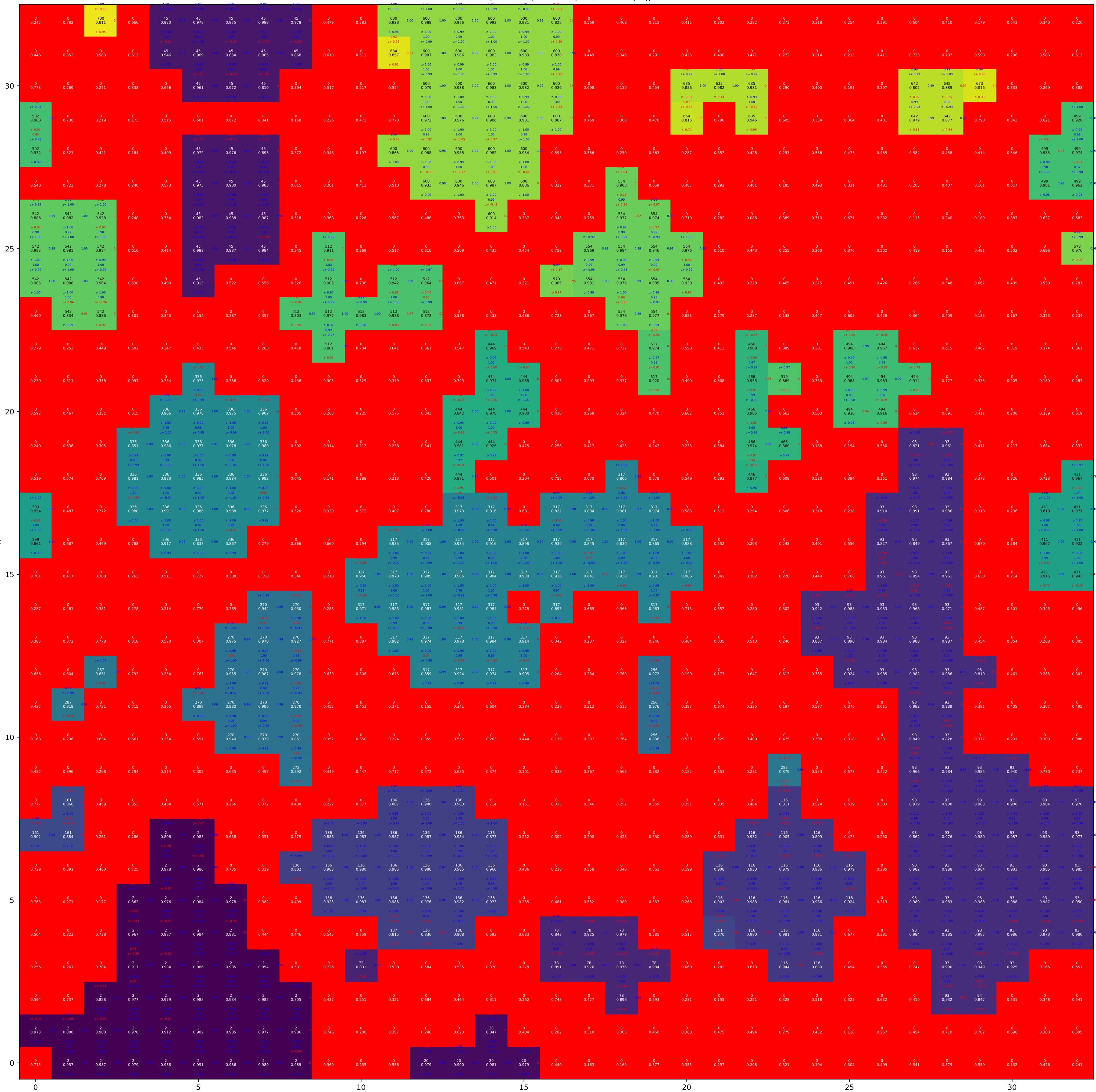
Cluster labels, PVA-300, T = 0.88, Tdot = 10**(-3), z = 11
