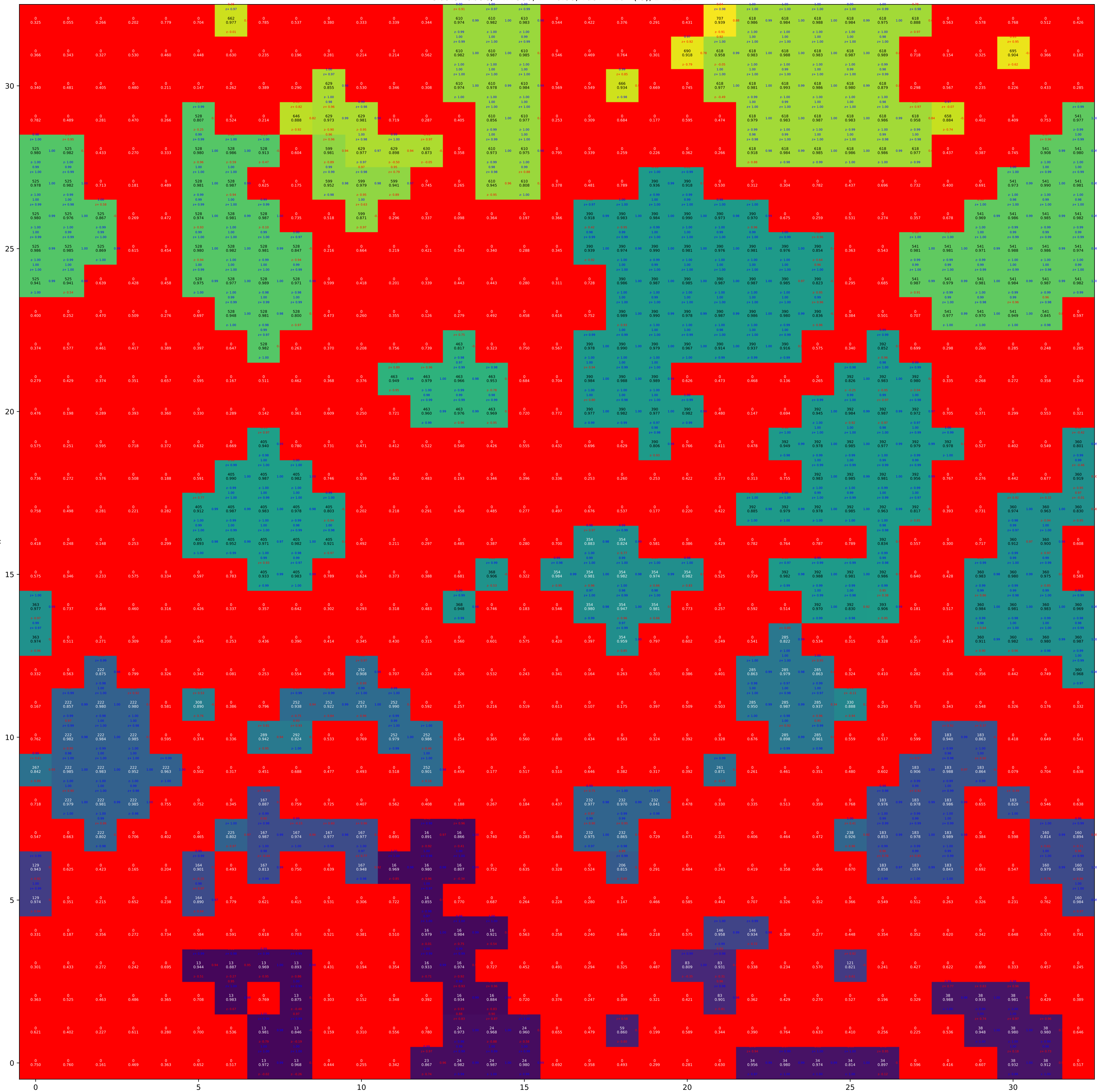
Cluster labels, PVA-300, T = 0.88, Tdot = 10*(-3), z = 22
