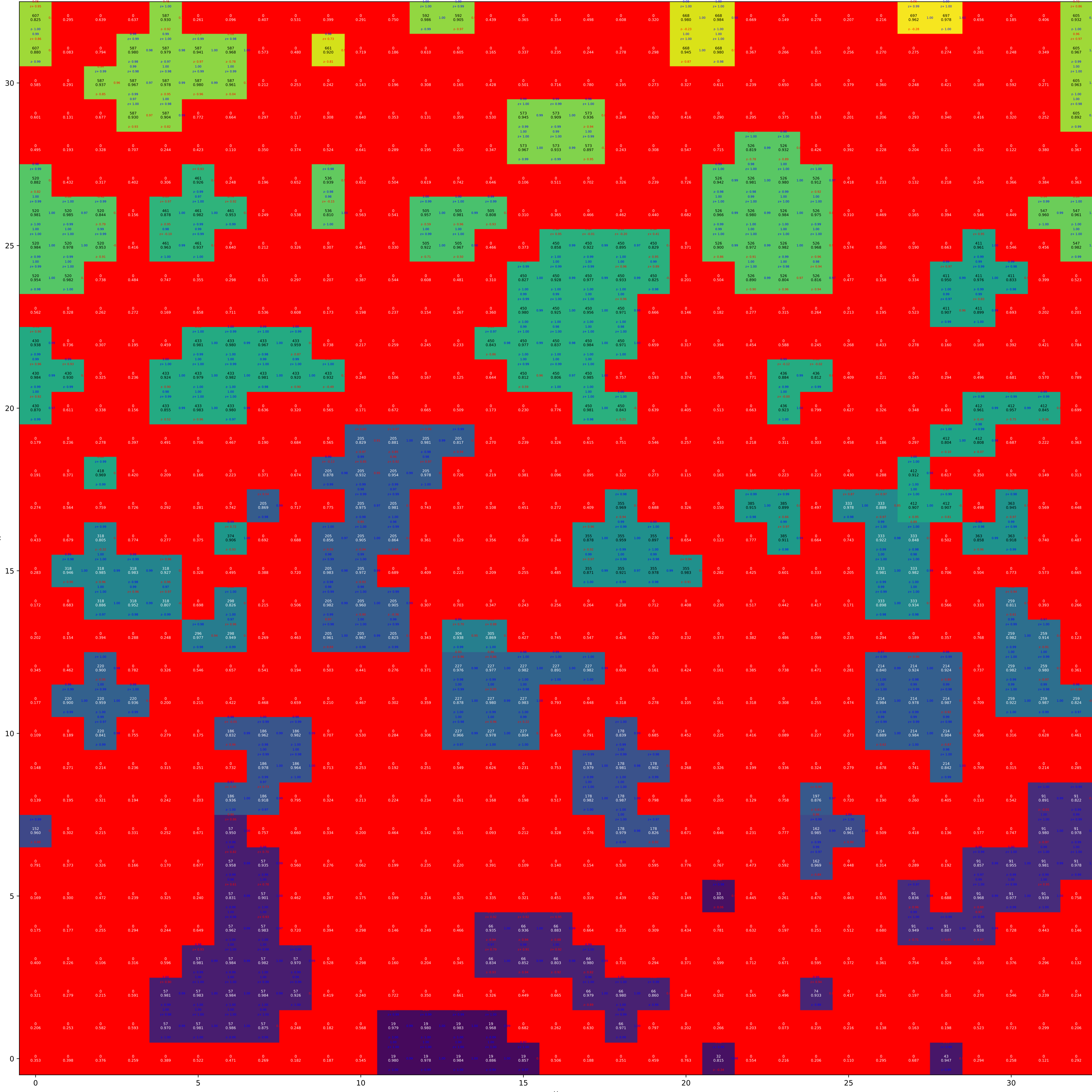
Cluster labels, PVA-500, T = 0.88, Tdot = 10**(-3), z = 24
