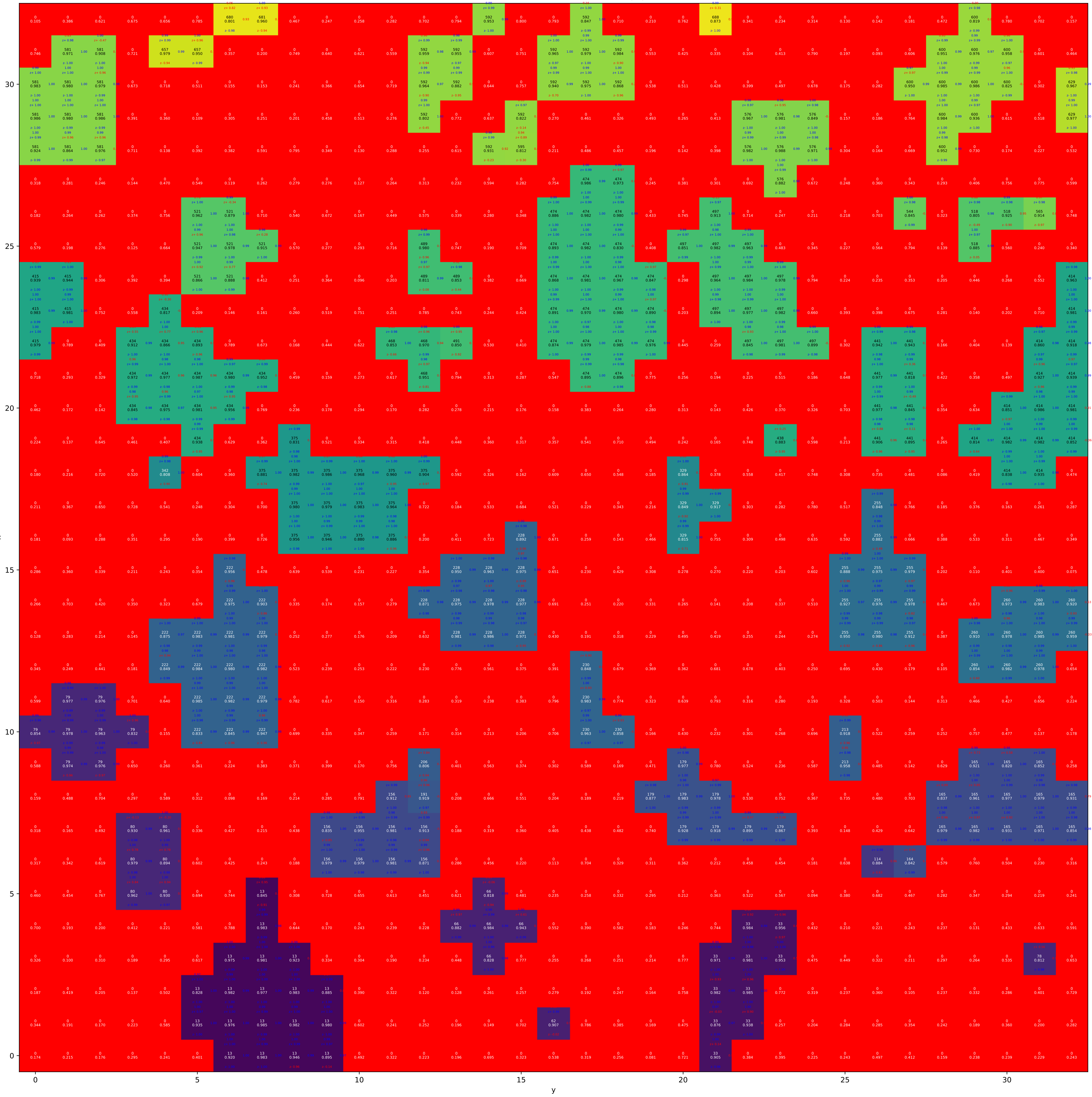
Cluster labels, PVA-500, T = 0.88, Tdot = 10**(-3), z = 30
