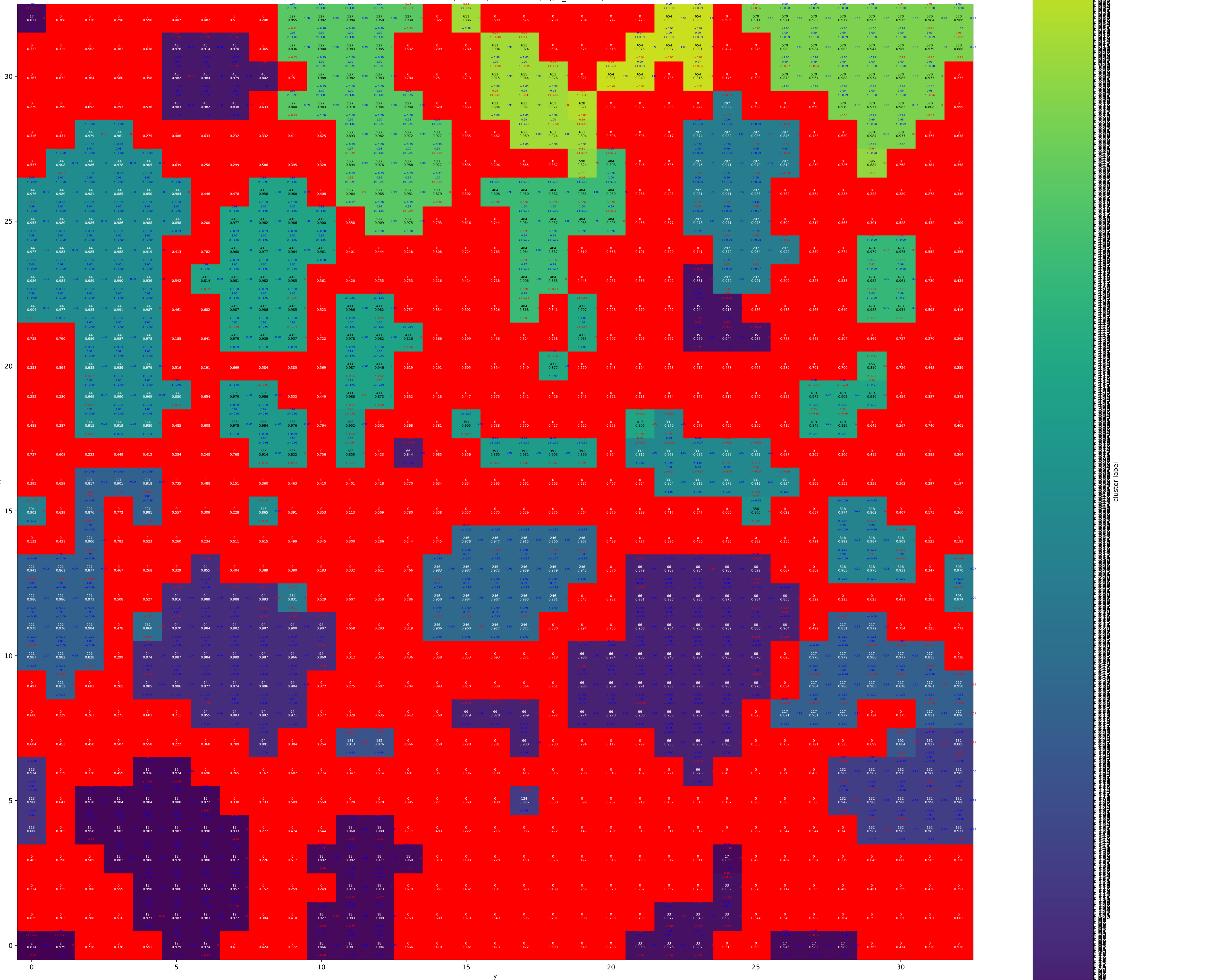
Cluster labels, PVA-100, T = 0.5, Tdot = 10*(-5), T_init = 1.0, z = 8
