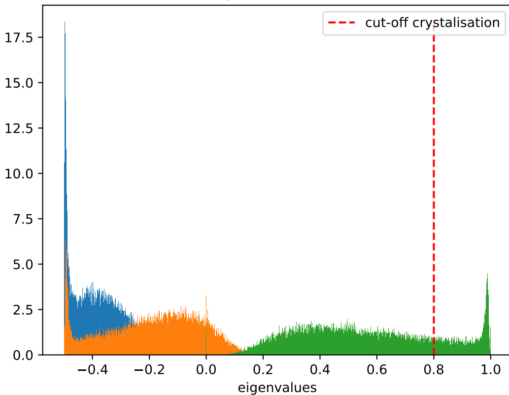
Distribution of eigenvalues at T = 0.5 , \dot{T} = 10^{-5}
