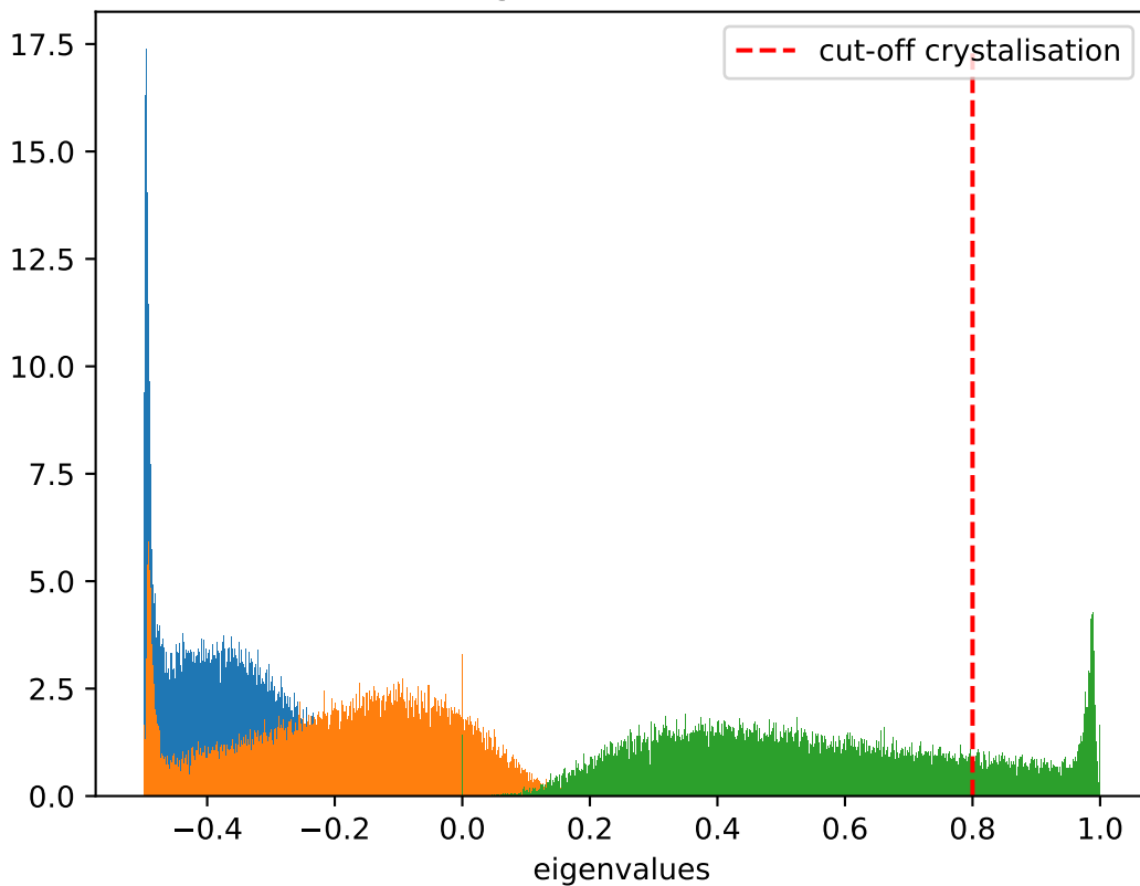
Distribution of eigenvalues at T = 0.55 , \dot{T} = 10^{-5}
