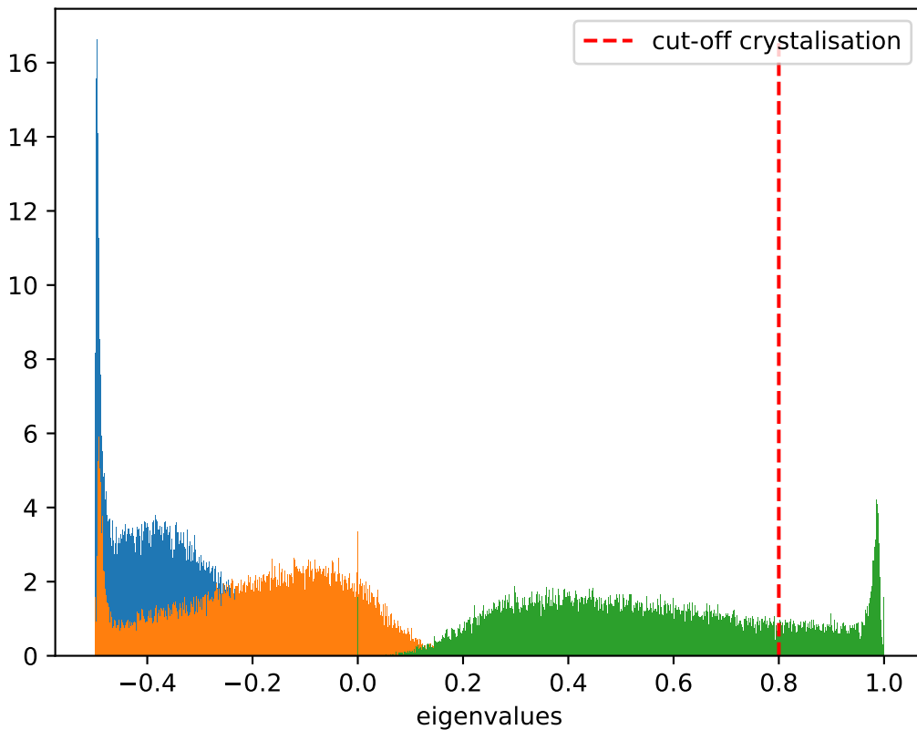
Distribution of eigenvalues at T = 0.575 , \dot{T} = 10^{-5}
