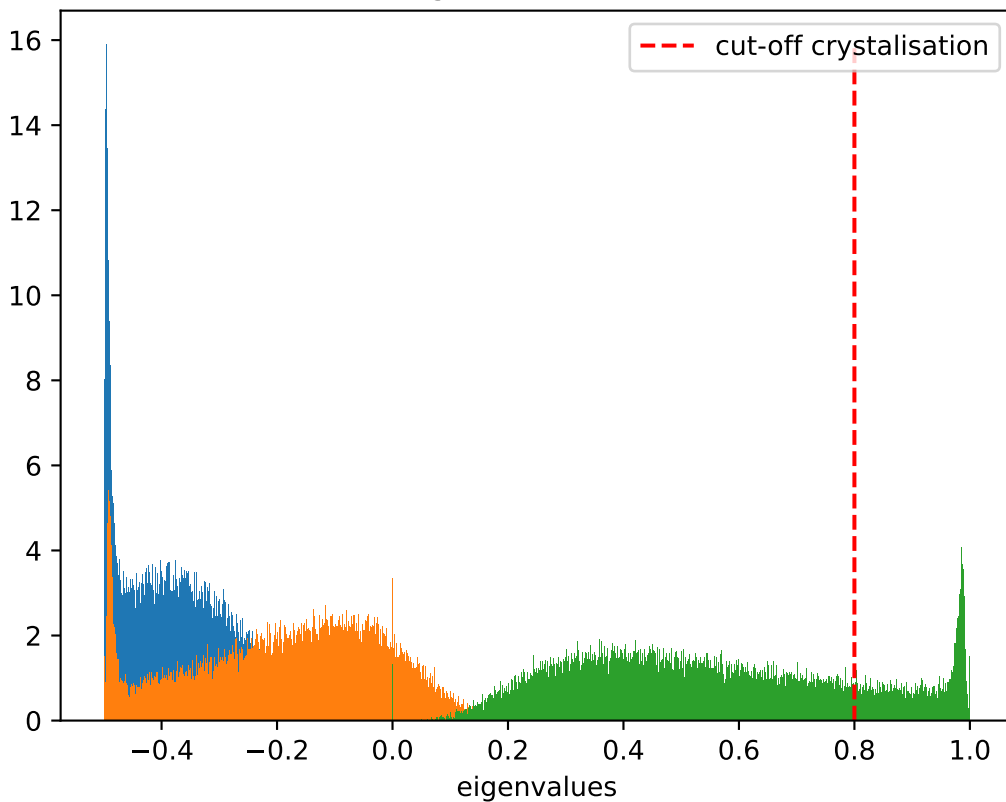
Distribution of eigenvalues at T = 0.6 , \dot{T} = 10^{-5}
