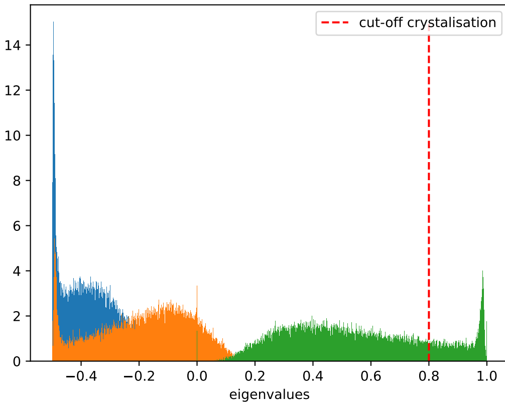
Distribution of eigenvalues at T = 0.625 , \dot{T} = 10^{-5}
