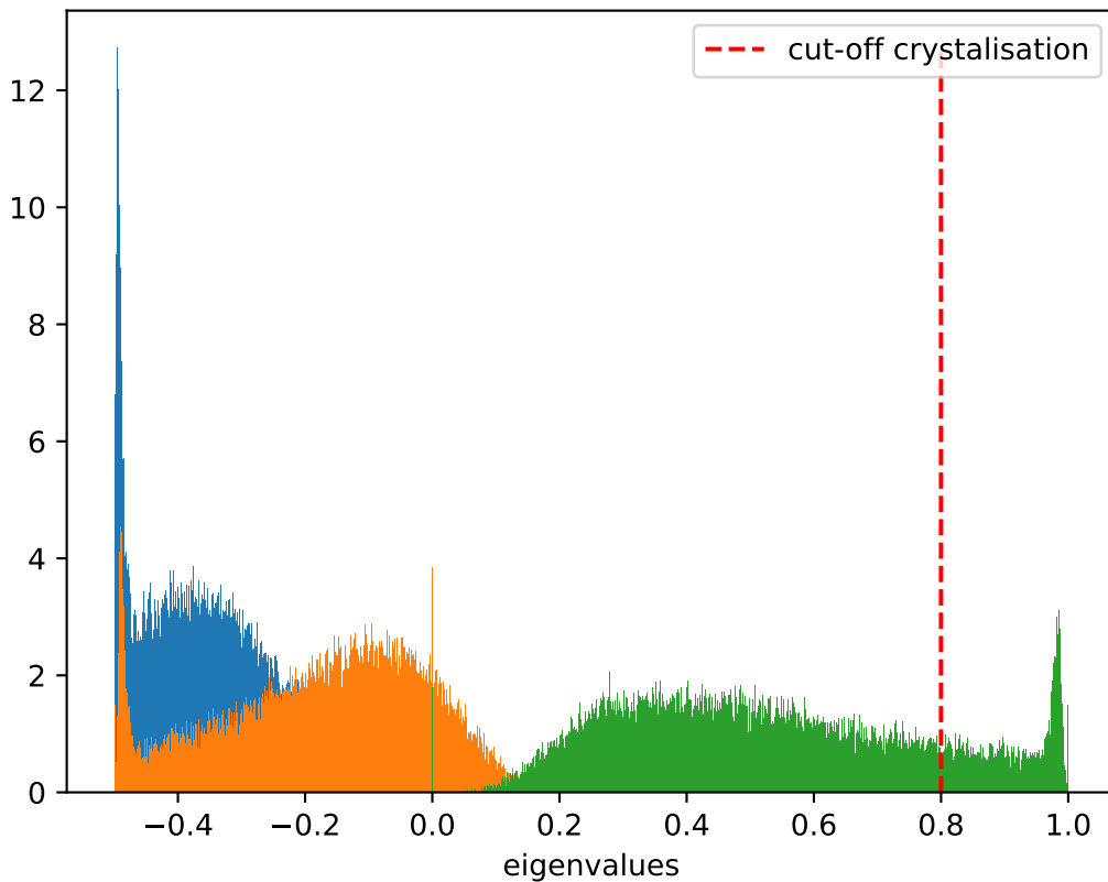
Distribution of eigenvalues at T = 0.7 , \dot{T} = 10^{-5}
