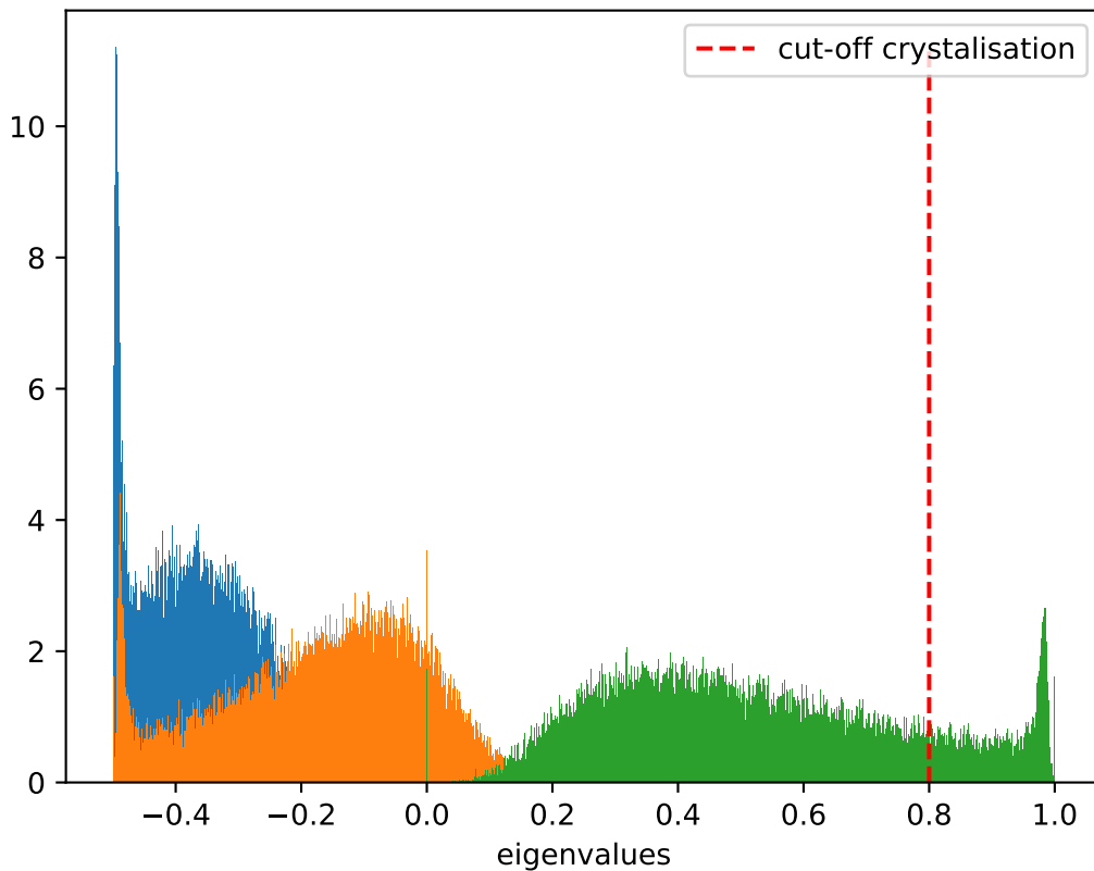
Distribution of eigenvalues at T = 0.725 , \dot{T} = 10^{-5}
