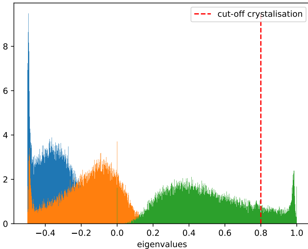
Distribution of eigenvalues at T = 0.75 , \dot{T} = 10^{-5}
