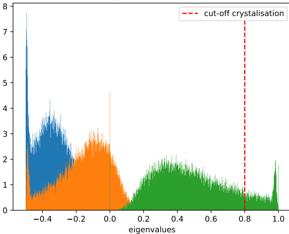
Distribution of eigenvalues at T = 0.775 , \dot{T} = 10^{-5}
