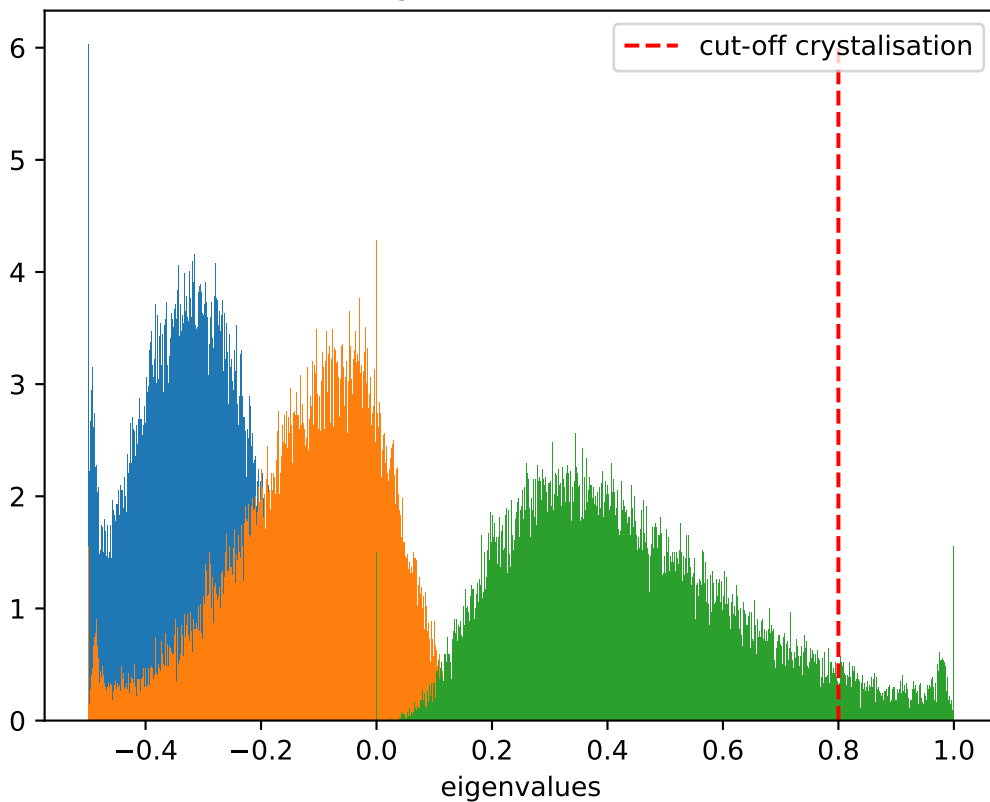
Distribution of eigenvalues at T = 0.825 , \dot{T} = 10^{-5}
