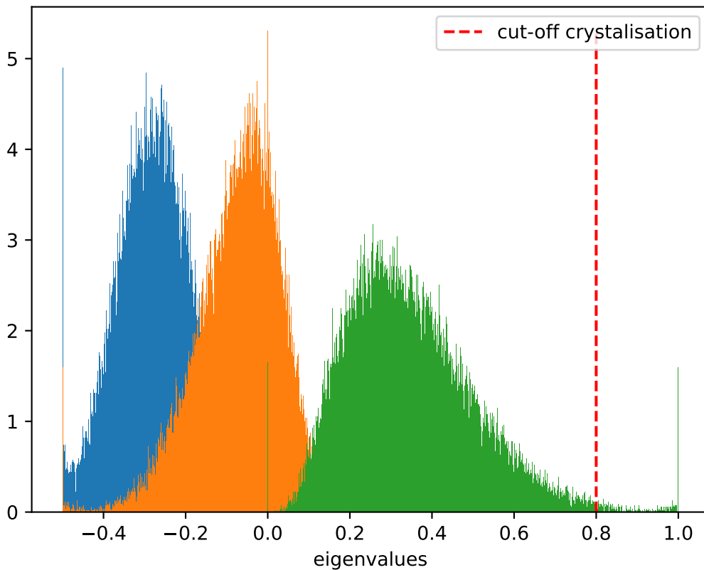
Distribution of eigenvalues at T = 0.9 , \dot{T} = 10^{-5}
