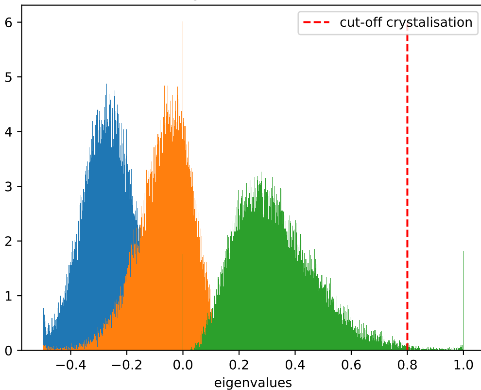
Distribution of eigenvalues at T = 0.925 , \dot{T} = 10^{-5}
