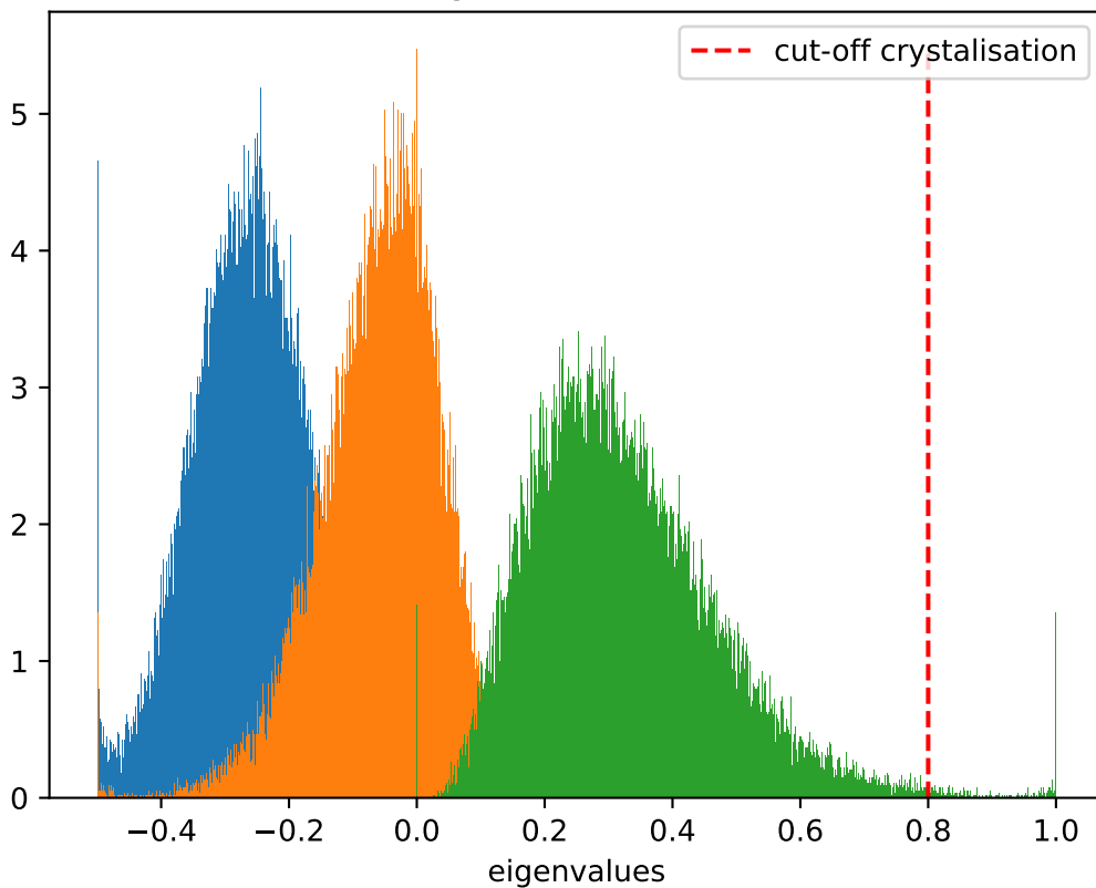
Distribution of eigenvalues at T = 0.95 , \dot{T} = 10^{-5}
