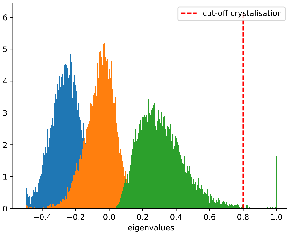
Distribution of eigenvalues at T = 0.975 , \dot{T} = 10^{-5}
