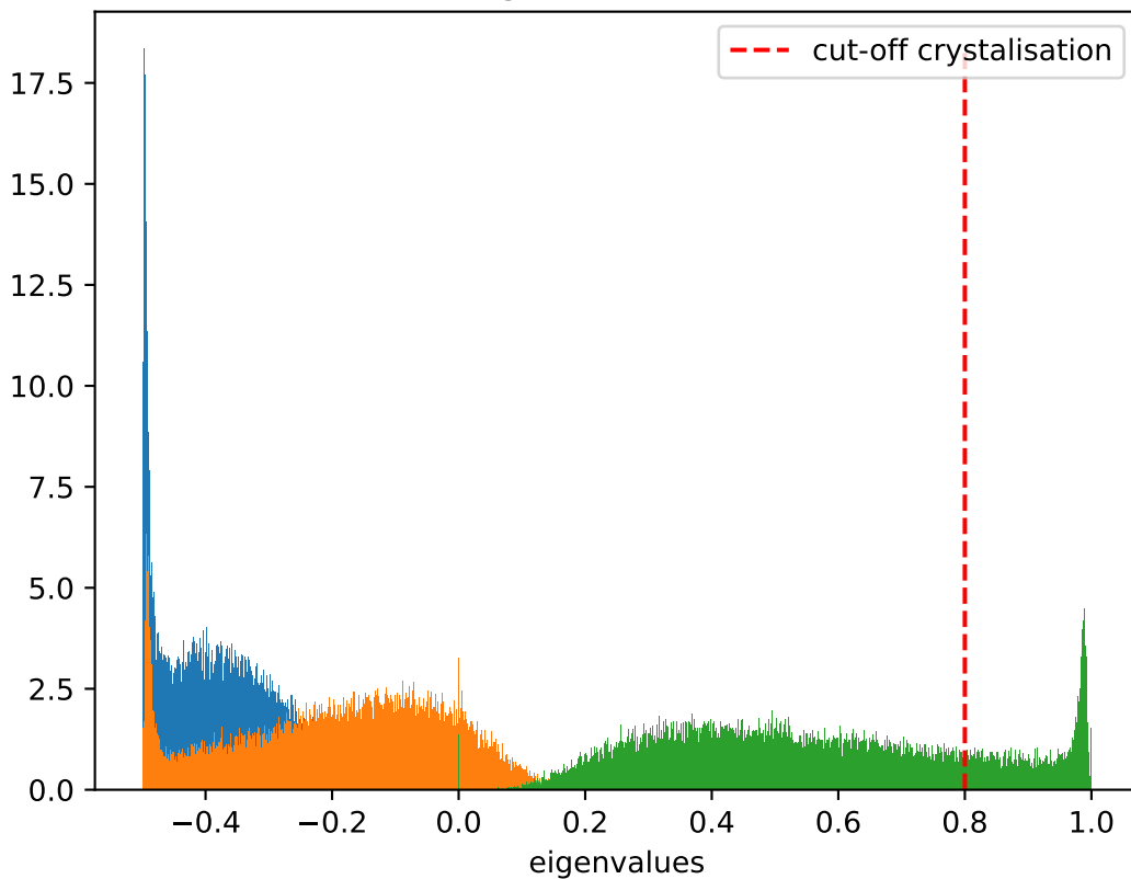
Distribution of eigenvalues at T = 0.5 , \dot{T} = 10^{-7}
